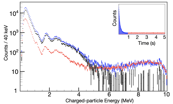
FIG. 6. Illustration of the component spectra and procedure used to obtain the ^{71}\text{Kr} background-subtracted charged-particle spectrum. Charged-particle spectra of decay events correlated within 1 s after implantation (blue) and a time normalized charged-particle spectrum of events correlated between 1–5 s after implantation (red) are shown. The inset shows a schematic representation of the events used in the background subtraction procedure. Residual (black) of the two spectra showing charged particles from ^{71}\text{Kr} \beta decay.
