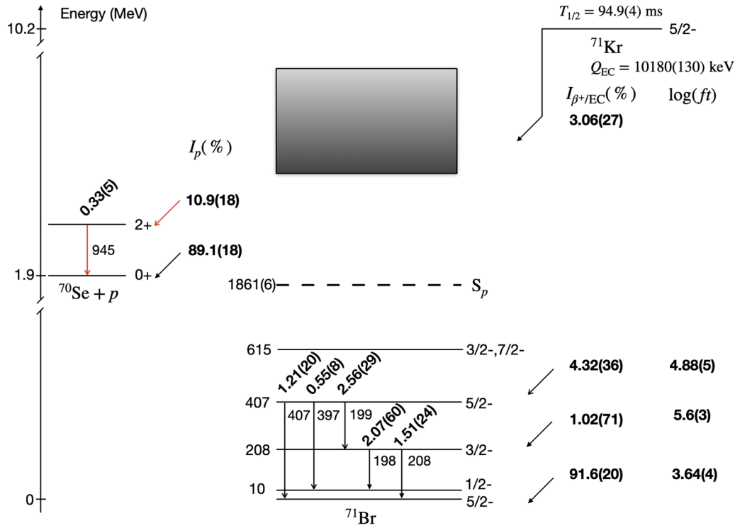
FIG. 8. Deduced \beta -delayed proton decay scheme of ^{71}\text{Kr} . Absolute intensities per 100 decays are given for the \gamma -ray transitions corrected for internal conversion, I_{(\gamma+ec)} , where the internal conversion coefficients were calculated using BrIcc assuming pure M1 transitions except for the 397-keV 5/2^- \rightarrow 1/2^- transition where pure E2 was assumed. Proton-unbound states (continuum of states) in ^{71}\text{Br} are denoted as a shaded rectangle. The newly observed feeding to the excited state in ^{70}\text{Se} in this experiment is shown in red (open arrow). Absolute \beta^+/EC intensities, I_{\beta^+/EC} , and \log(ft) values should be taken as limits when considering possible unobserved feeding. If pure E2 transitions are assumed, the branching intensities to the 407-keV, 207-keV, and g.s. levels are 4.61(33)%, 0.77(74)%, and 91.6(20)%, respectively. Q_{EC} and S_p obtained from Ref. [30].
