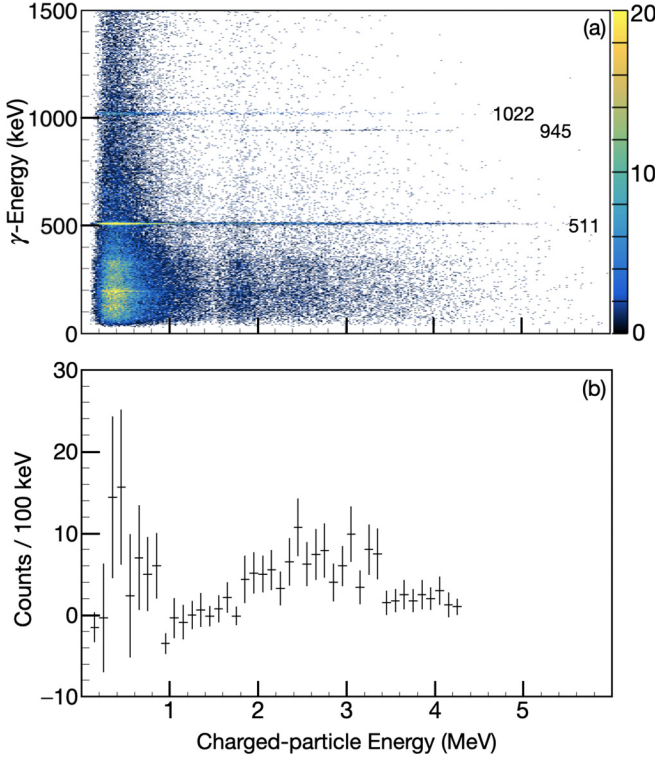
FIG. 7. Examination of charged particles coincident with \gamma rays following the decay of ^{71}\text{Kr} . Background-subtracted (a) \gamma -ray energy versus charged-particle energy matrix for ^{71}\text{Kr} \beta decay and (b) charged-particle energy spectrum in coincidence with 945-keV \gamma rays. The 945-keV \gamma ray is in coincidence with charged-particle energies from 1.5 to 5.0 MeV. The color scale represents the number of counts.
