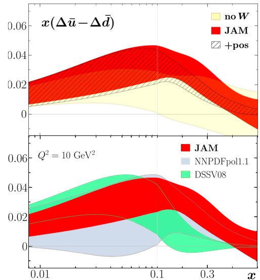
FIG. 2. Polarized sea quark asymmetry x(\Delta\bar{u} - \Delta\bar{d}) from JAM (red 1\sigma bands) at Q^2 = 10 GeV 2 compared with: [top panel] fit without RHIC W/Z data (yellow band) and the result with positivity constraints (hatched band), and [bottom panel] the NNPDFpol1.1 [50] and DSSV08 [48] analyses.
