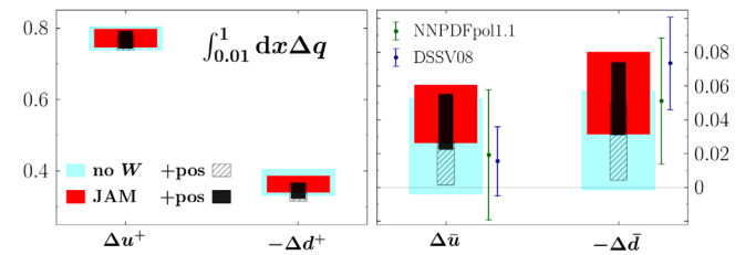
FIG. 4. Truncated integrals \int_{0.01}^1 dx \Delta q(x) at Q^2 = 4 \text{ GeV}^2 for \Delta u^+ , -\Delta d^+ , \Delta\bar{u} and -\Delta\bar{d} from this analysis (red rectangles) compared with the fit without the RHIC W/Z data (cyan) and with positivity constraints (small hatched squares without RHIC and black squares with RHIC). For the antiquarks, NNPDFpol1.1 (green points) and DSSV08 (blue points) are also shown. The vertical height of the bands represents 1\sigma uncertainty.
