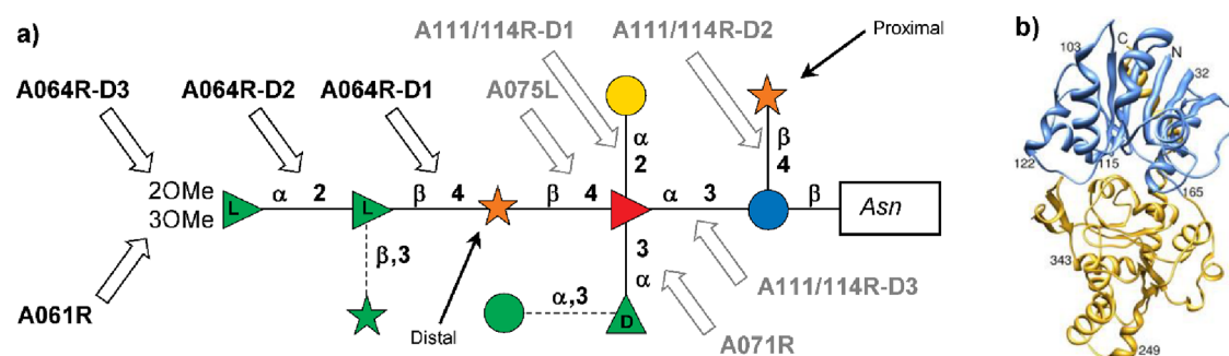
Figure 15. Comprehensive view of PBCV-1 GTs. (a) Structure of PBCV-1 N-glycan with known and predicted GTs activities. Text in black indicates that the activity has been experimentally validated, otherwise (text in gray) the activity was deduced by indirect evidence. (b) Crystallographic structure of B736L (PDB 3OY2) from the chlorovirus NY-2A, which shares high conservation with A546L of PBCV-1, whose activity is yet to be uncharacterized. Reproduced with permission from ref 213. Copyright 2010 American Society for Microbiology.
