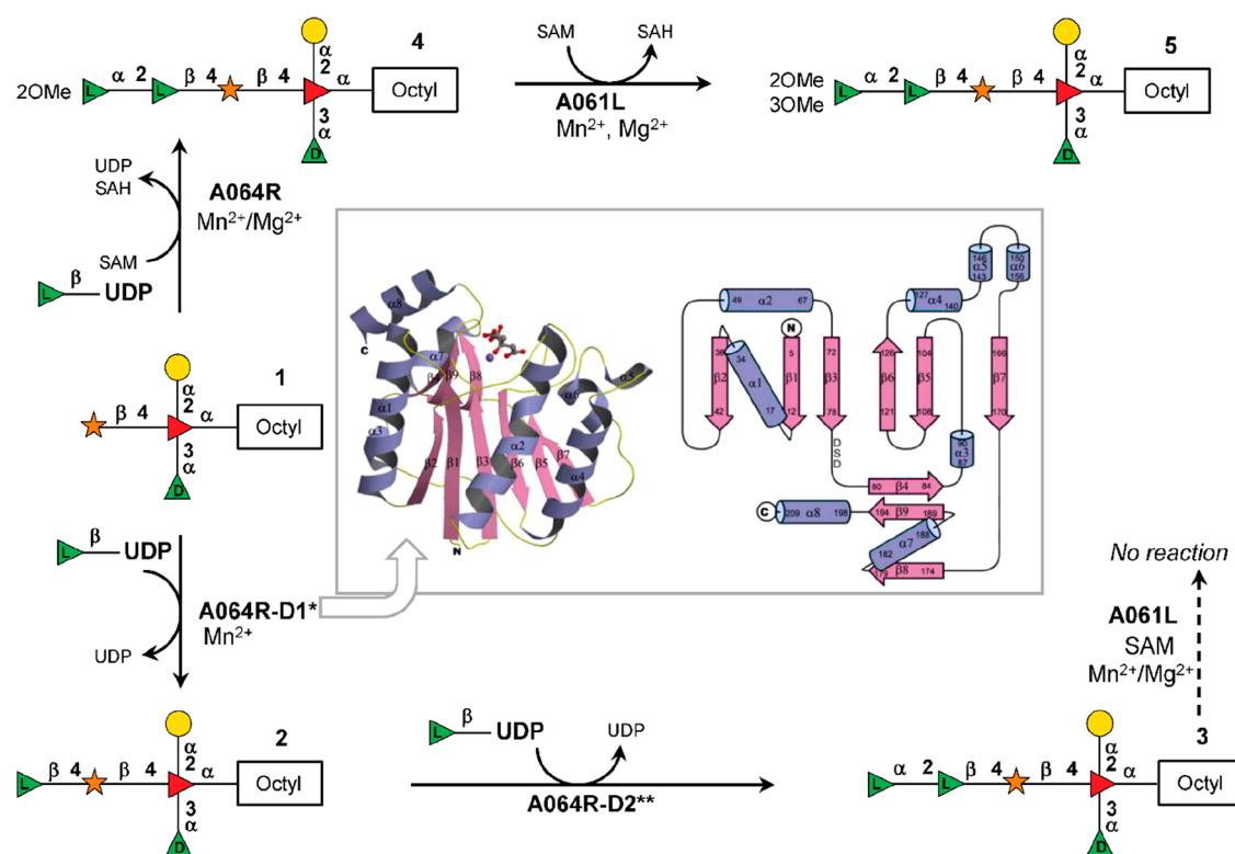
Figure 14. Biochemical assays of A064R and its individual domains. Substrate 1 was used as an analogue of the N-glycan from a class B variant (Figure 13), and it was transformed into 2 by A064R-D1 and, in turn, converted into 3 by A064R-D2. Substrate 1 was used to assess the activity of the complete A064R and validated domain 3 as responsible for adding a methyl group to the O-2 position of the terminal L-Rha. Product 4 (but not 3) was the substrate for A061L, which added the methyl to O-3 of the terminal L-Rha. The inset at the center displays the crystallographic structure of A064R-D1 and the sequence of the secondary structural motifs. Adapted with permission from ref 142. Copyright 2007 Elsevier. *A064R-D1 could also use Xyl as a substrate. **A064R-D2 could also use Rha as a substrate.
