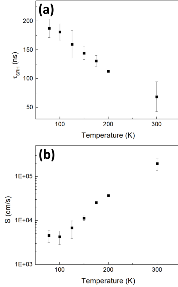
Figure 5: Temperature-dependence of (a) \tau_{SRH} , and (b) S , for Ba 3 Zr 2 S 7 determined from the data and models shown in Fig 4.
