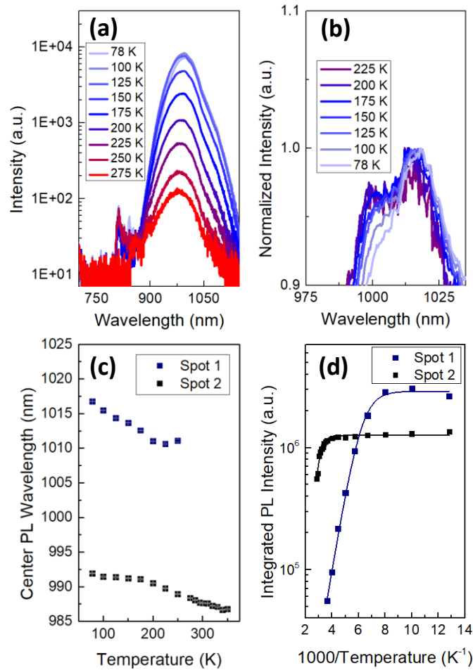
Figure 2: Steady-state PL results measured with an excitation wavelength of 705 nm on a Ba 3 Zr 2 S 7 single-crystal. (a) Temperature-dependent spectra, plotting the absolute measured intensity. (b) Temperature-dependent spectra, plotting spectrally-corrected, normalized intensity. (c-d) Analysis of the temperature-dependent PL spectra, for two measurement spots, the first of
