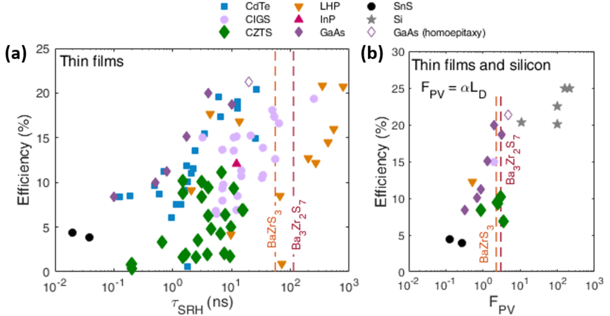
Figure 6: SRH lifetime ( \tau_{SRH} ) and solar cell figure of merit F_{PV} = \alpha L_D vs. energy conversion efficiency for various photovoltaic materials. BaZrS_3 and Ba_3Zr_2S_7 are plotted as dashed lines corresponding to the best-estimates of our TRPL data analysis; no solar cells of either material have yet been reported. In (a), we only show data for which \tau_{SRH} and device measurements were performed on samples that were synthesized in the same laboratory and using as close to the same procedure as is reasonably possible; in (b), we additionally require that D and \alpha are reported on comparable samples, with the exception of silicon and GaAs for which we use tabulated values. Data are adapted from refs. 28,30–32
