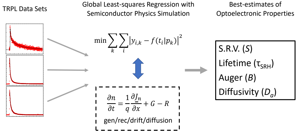
Figure 1: Flow chart of TRPL data analysis. Multiple data sets are acquired at a given temperature with varying pump fluence and/or wavelength. The data are modeled using a generation-recombination-drift-diffusion solver in one spatial dimension, and the model is refined using global least-squares minimization of all data sets (indexed by k ) with customizable parameter sets ( p_k ). The results are best-estimates of properties such as surface recombination velocity ( S ), non-radiative recombination lifetime ( \tau_{SRH} ), and ambipolar diffusivity ( D_a ) that are directly relevant to optoelectronic performance.
