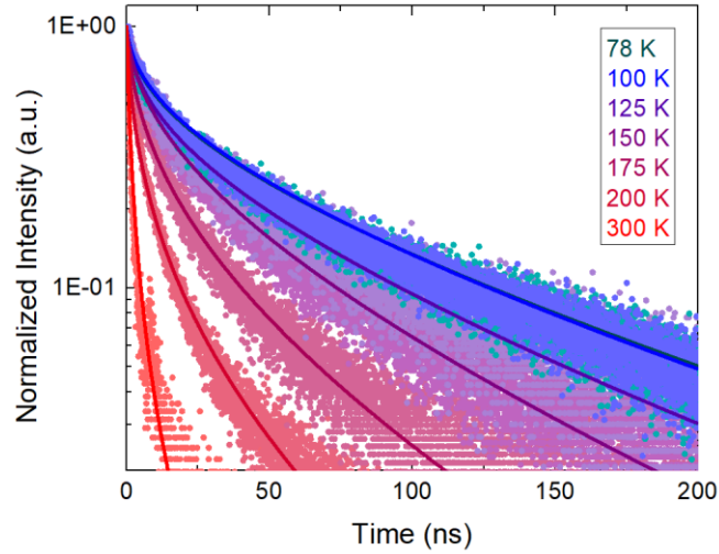
Figure 4: TRPL spectra measured on a Ba 3 Zr 2 S 7 crystal for temperature between 78 and 300 K, measured with pump wavelength 705 nm and pump of 3.85 mJ/cm 2 ( 1.37 \times 10^{16} ph/cm 2 ) per pulse. The TRPL data (points) and best-fit models (lines) are normalized to accentuate the rise in decay rate with increasing temperature.
