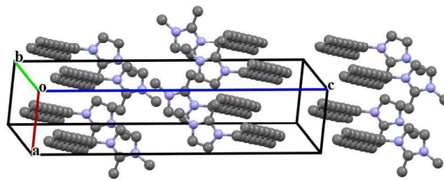
Fig. 3 Representative packing diagram for the cations of compound 2 showing the alternating alignment of the alkyl groups. Hydrogens and bromine atoms are omitted for clarity.
