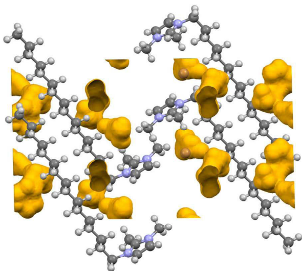
Fig. 11 Depiction of void spaces (yellow) in the structure of 2 .
