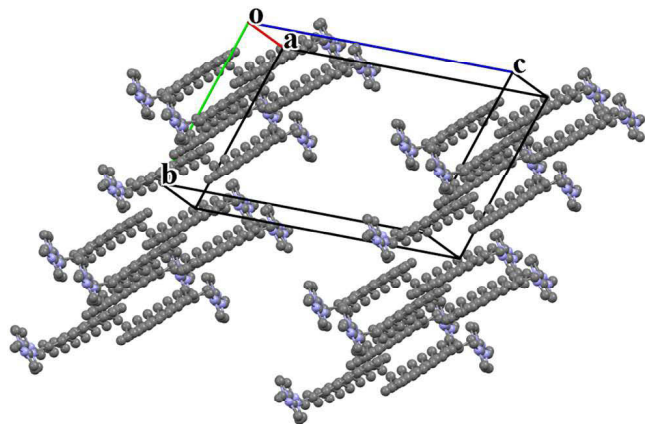
Fig. 7 Representative packing diagram for the cations in compound 4 showing the interdigitated alkyl groups. Hydrogen atoms, \text{Tf}_2\text{N}^- anions are omitted for clarity. Both disordered portions of the cations are shown.
