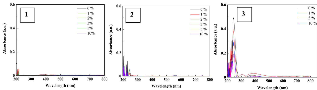
Fig. 17 UV-vis spectra of compounds 1–3 in mixtures of methanol:chloroform. Percentages refer to methanol.
