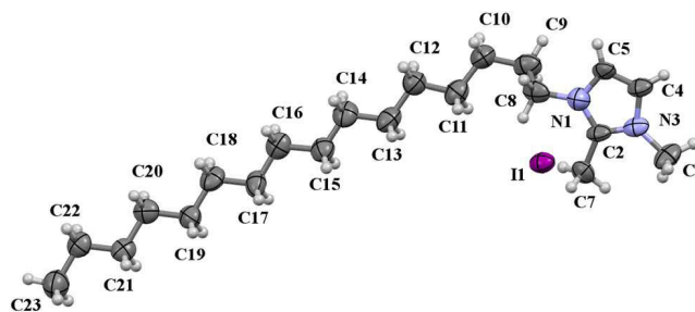
Fig. 4 Asymmetric unit of 3 shown with 50% probability ellipsoids. Gray = carbon, white = hydrogen, blue = nitrogen, purple = iodine.
