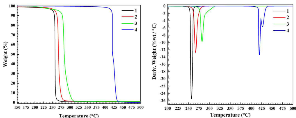
Fig. 13 Thermal decomposition traces for compounds 1–4 (left) and the derivative curves (right).
