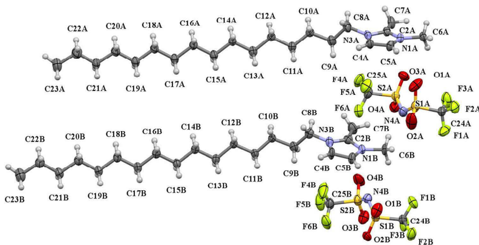
Fig. 6 Asymmetric unit of 4 shown with 50% probability ellipsoids. Disordered parts C and D omitted for clarity. Gray = carbon, white = hydrogen, blue = nitrogen, red = oxygen, green = fluorine, yellow = sulfur.
