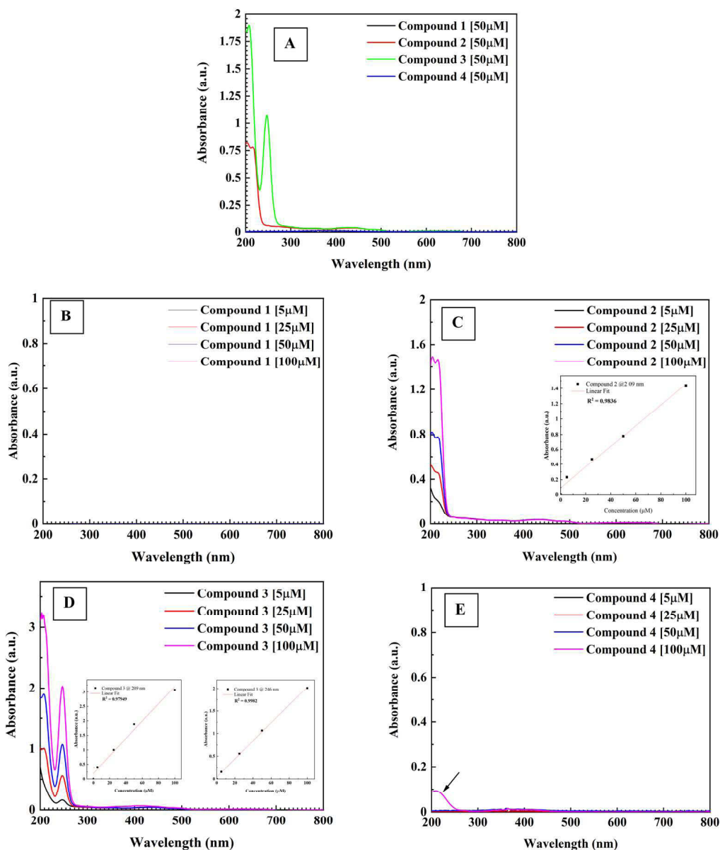
Fig. 16 (A) UV-vis spectra for compounds 1–4 at 50 \mu\text{M} concentration in acetonitrile. (B–E) UV-vis concentration studies for compounds 1–4 in acetonitrile.
