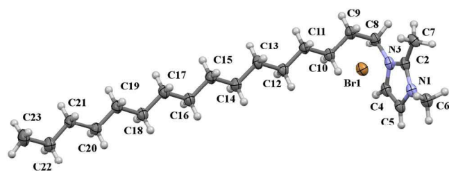
Fig. 2 Asymmetric unit of 2 shown with 50% probability ellipsoids. Gray = carbon, white = hydrogen, blue = nitrogen, tan = bromine.
