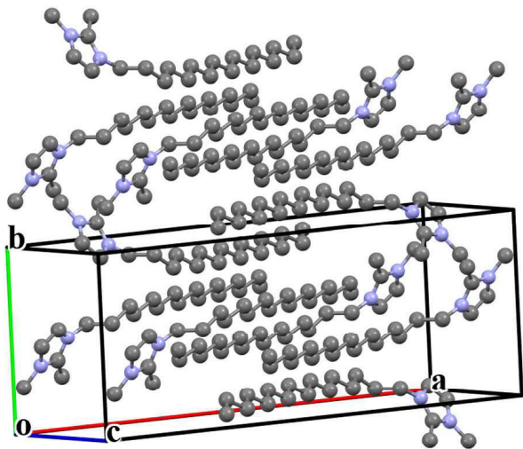
Fig. 5 Representative packing diagram for the cations of compound 3 showing the interdigitated alkyl groups. Hydrogens and iodide atoms are omitted for clarity.
