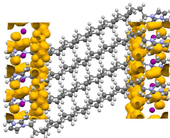
Fig. 12 Depiction of void spaces (yellow) in the structure of 3 .
