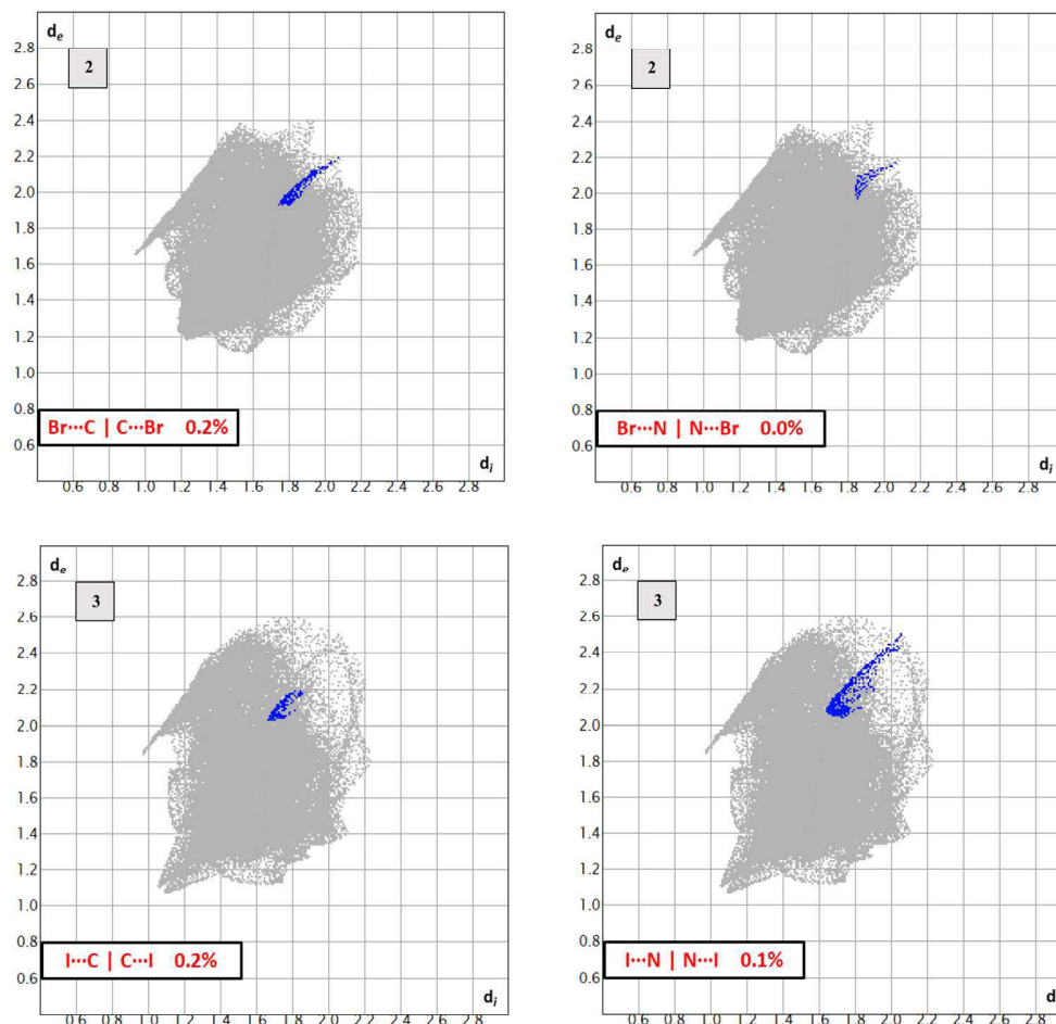
Fig. 10 Fingerprints for 2 and 3 showing the negligible anion \cdots\pi interactions in the crystals.
