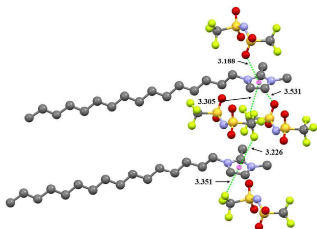
Fig. 9 Depiction of anion... \pi interactions in 4. Hydrogens and disorder are omitted for clarity. Distances are shown in angstroms to the centroid of the rings.
