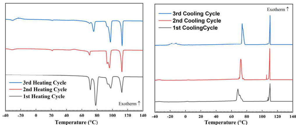
Fig. 15 Traces of the three consecutive heating cycles (left) and cooling (right) for compound 3 . Y axis is offset for clarity.
