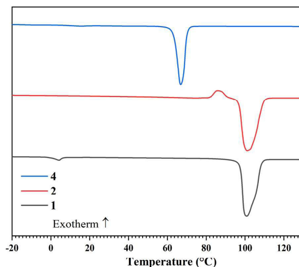
Fig. 14 DSC traces for compounds 1 , 2 , and 4 taken from the 2nd heating cycle for each compound. Y axis is offset for clarity.
