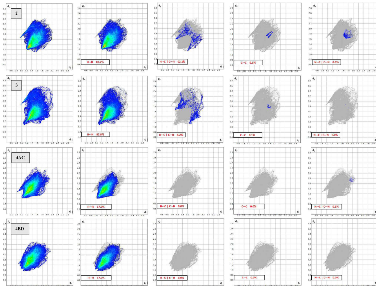
Fig. 8 Fingerprints for compounds 2–4 showing important intermolecular interactions of the cations.
