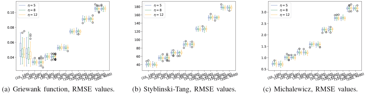
Figure 4: RMSE (y-axis) as a function of dimensionality and sample size (d, n) (x-axis) for SGPMA.
