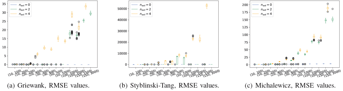
Figure 2: RMSE (y-axis) as a function of dimensionality and sample size (d, n) (x-axis) for GE-KPLS.
