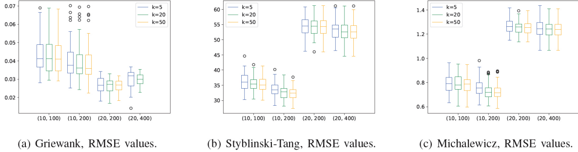
Figure 6: RMSE (y-axis) as a function of dimensionality, sample size (d, n) (x-axis) for GPMCMC.
