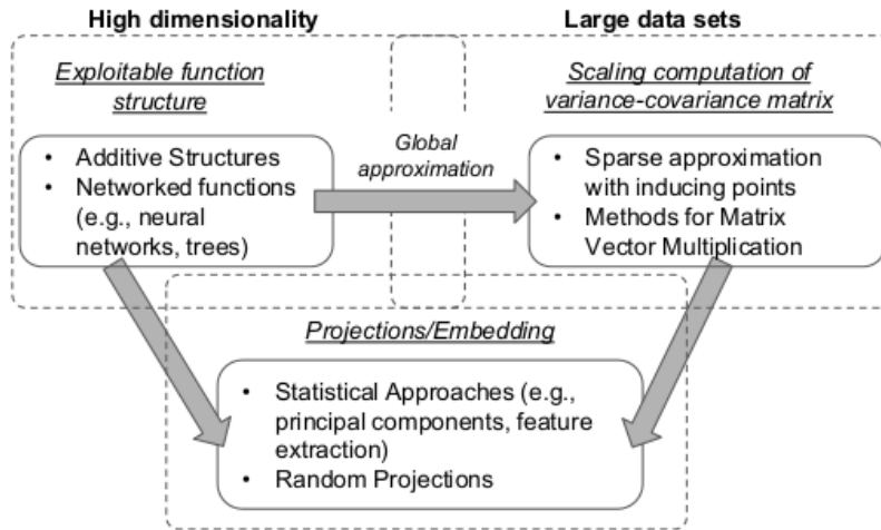
Figure 1: Graphical representation for the classification dimensions.
