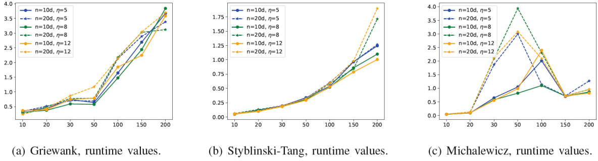
Figure 5: Runtime (y-axis) as a function of dimensionality d (x-axis) for SGPMA.
