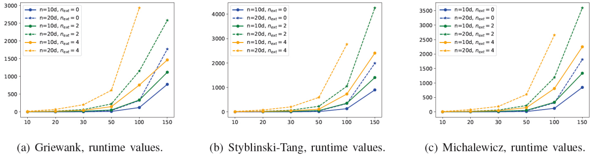
Figure 3: Runtime (y-axis) as a function of dimensionality d (x-axis) Performance for GE-KPLS.
