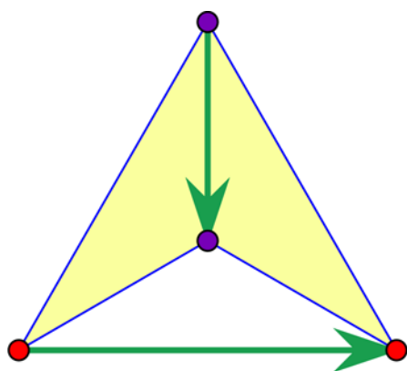
Figure 3. Deforming the quadrilateral in Figure 2.
