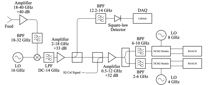
Fig. 2. Signal path for the WVR. The signals from the 18–26 GHz spectral and 28–30 GHz continuum channels are processed separately. For the detailed schematics of signal processing with the downconverter module (‘DCM2’), see Fig. 2 in [3].
