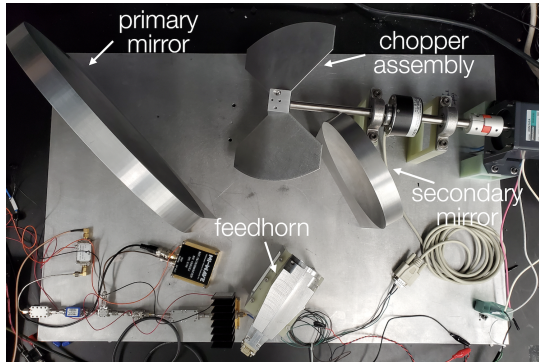
Fig. 1. The WVR assembly under test in the lab. The optical and mechanical elements comprising the WVR system are indicated. We will design a new enclosure with heated and ambient calibration loads installed for mounting onto the telescope.
