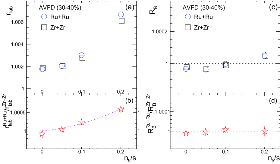
Fig. 8. (color online) r_{\text{lab}} (a) and R_B (c) as a function of n_s/s from the EBE-AVFD model for the 30%-40% Ru+Ru and Zr+Zr collisions at \sqrt{s_{NN}} = 200 GeV, with their ratios between Ru+Ru and Zr+Zr in panels (b) and (d), respectively. In panel (b), the 2 nd -order-polynomial fit function demonstrates the rising trend starting from (0, 1).
