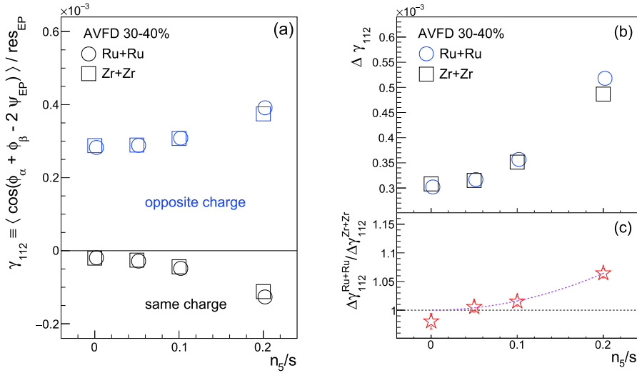
Fig. 4. (color online) EBE-AVFD calculations of \gamma_{112}^{OS(SS)} (a) and \Delta\gamma_{112} (b) as functions of n_5/s for the 30%-40% isobar collisions at \sqrt{s_{NN}} = 200 GeV, with the ratio of \Delta\gamma_{112} (c) between Ru+Ru and Zr+Zr. In panel (c), the 2 nd -order-polynomial fit function illustrates the rising trend starting from (0, 1).
