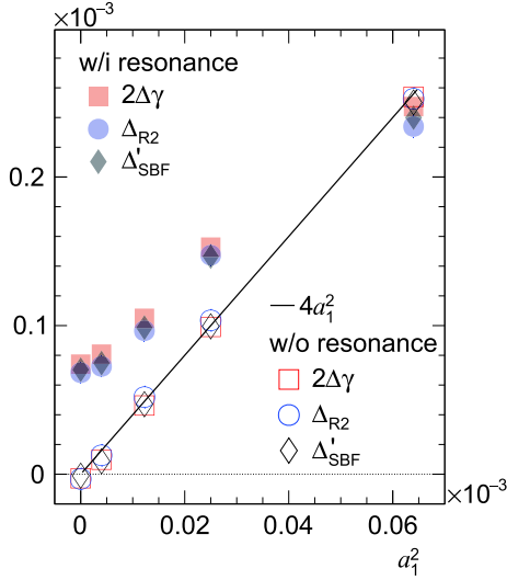
Fig. 2. (color online) The toy-model simulations of 2\Delta\gamma_{112} , \Delta_{R2} , and \Delta'_{SBF} \equiv \left( \frac{\pi^4}{64M^2} \Delta_{SBF} + \frac{8}{3} v_2 \Delta\delta \right) as a function of the input a_1^2 . The open markers represent the pure-signal scenario without resonances, and the solid markers denote the scenario with resonance decays. For comparison, the linear function of 4a_1^2 is also added.
