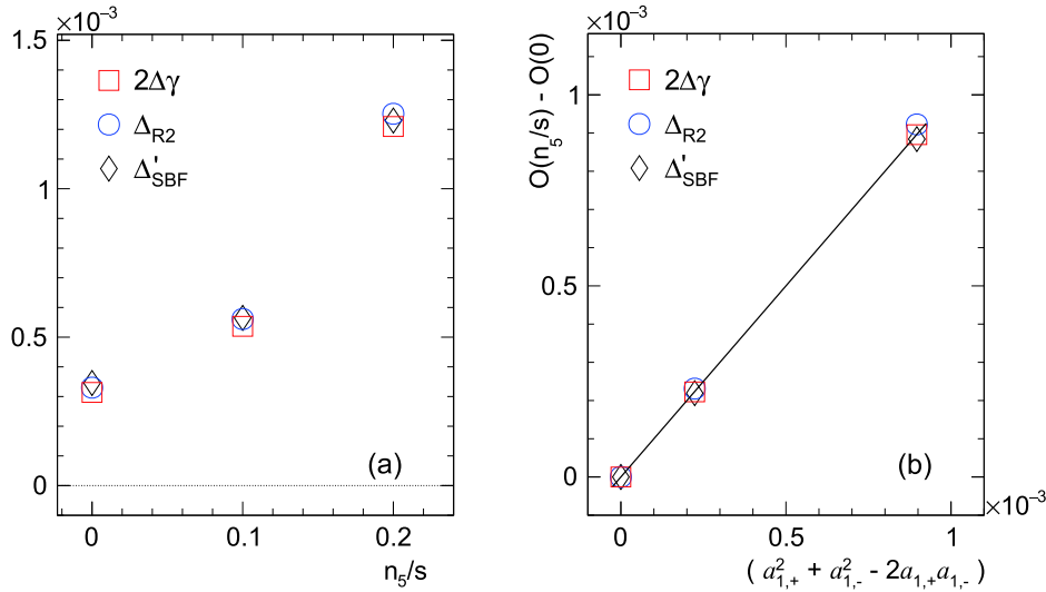
Fig. 3. (color online) (a) The EBE-AVFD simulations of 2\Delta\gamma_{112} , \Delta_{R2} , and \Delta'_{SBF} \equiv \left( \frac{\pi^4}{64M^2} \Delta_{SBF} + \frac{8}{3} v_2 \Delta\delta \right) as a function of n_5/s in the 30%-40% Au+Au collisions at 200 GeV. (b) The same results with the subtraction of the pure-background case vs (a_{1,+}^2 + a_{1,-}^2 - 2a_{1,+}a_{1,-}) . For comparison, a linear function of y = x is drawn to verify the relation in Eq. (39).
