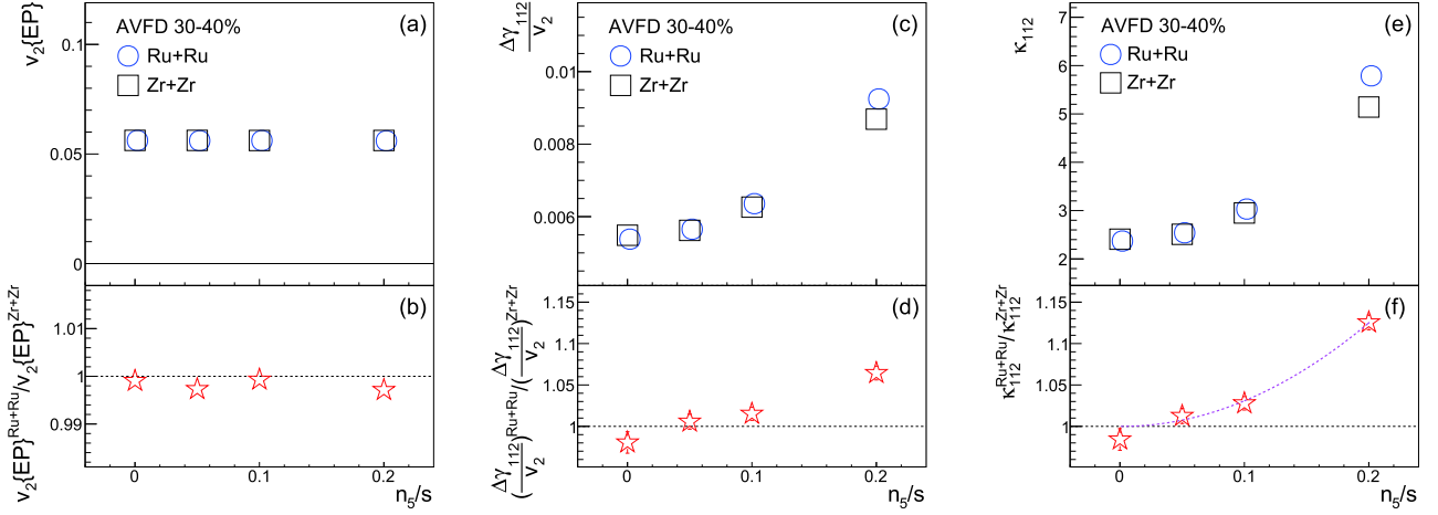
Fig. 6. (color online) EBE-AVFD calculations of v_2 (a), \Delta\gamma_{112}/v_2 (c), and \kappa_{112} (e) as functions of n_s/s for the 30%-40% isobar collisions at \sqrt{s_{\text{NN}}} = 200 GeV, with the ratios of v_2 (b), \Delta\gamma_{112}/v_2 (d), and \kappa_{112} (f) between Ru+Ru and Zr+Zr. In panel (f), the 2 nd -order-polynomial fit function illustrates the rising trend starting from (0, 1).
