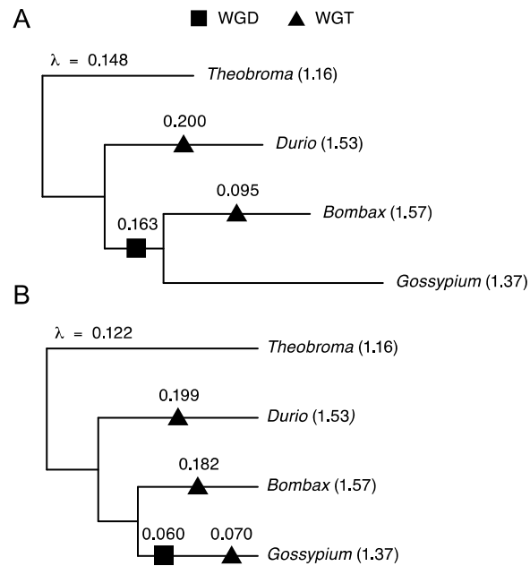
Figure 5. WGDgc results for gene count data and alternative models for the distribution of WGMs
