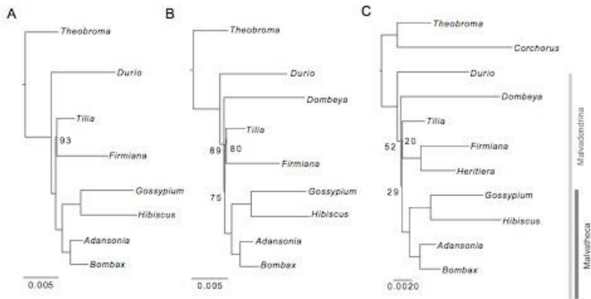
Figure 1. Maximum Likelihood trees based on the concatenated data sets of 67 plastid genes
