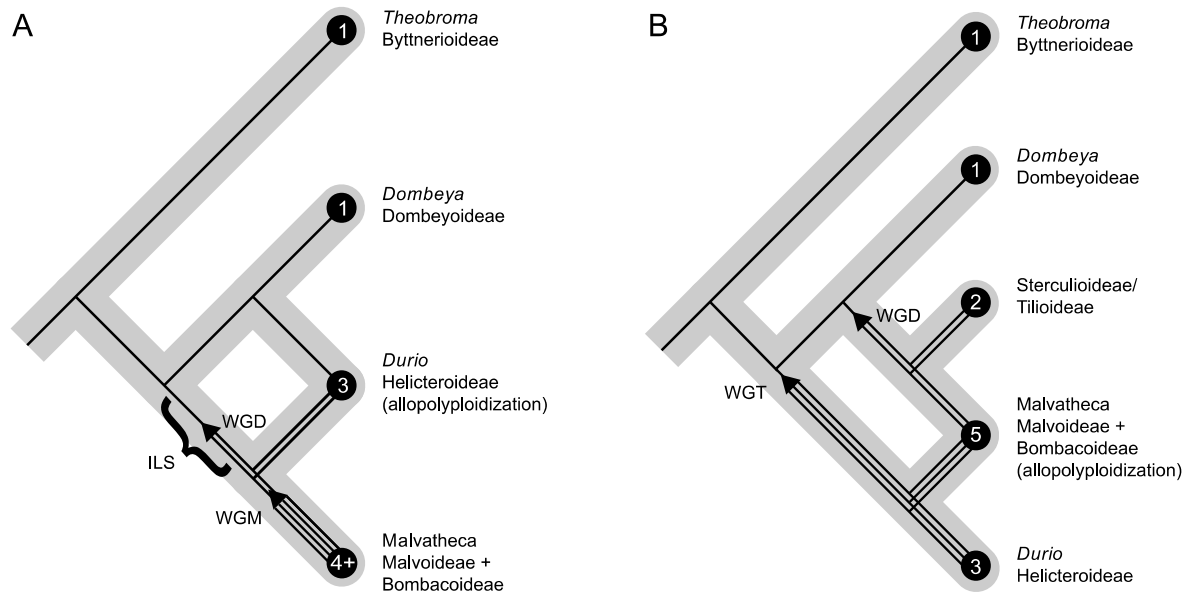
Figure 6. Hypotheses presented to explain the data
