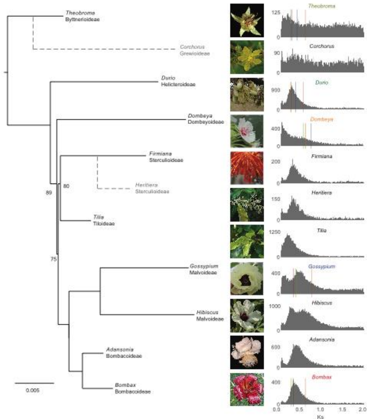
Figure 2. Malvaceae plastid phylogeny and Ks frequency histograms
