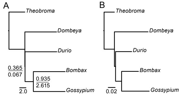
Figure 4. Phylogeny inferred by Bayesian concordance analysis of 1214 nuclear genes and maximum likelihood inference of concatenation of genes.
