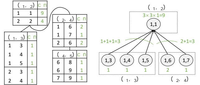
(a) Example database and final (b) Messages received and aggregated by an R -tuple.
