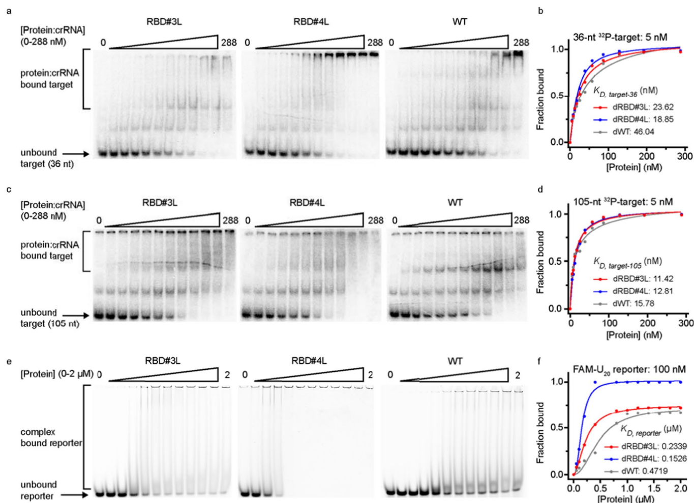
Extended Data Fig. 5 | Quantification of RNA binding with RBD#3L, RBD#4L, and WT LwaCas13a. a and c. Representative EMSA gel images of inactive HEPN2 mutants (R1046A/H1051A), that is, dRBD#3L, dRBD#4L, and dWT complexed with crRNA binding to 5 nM of body-radiolabeled ( ^{32}\text{P} ) target RNA. ( a , T26; c , T1). The protein:crRNA complex with a molar ratio of 1:0.95 was serially diluted to 288, 192, 128, 86, 57, 38, 25, 17, 12, 8 and 5 nM. The 0-nM control was target RNA with reaction buffer. b and d. Calculation of binding affinity between target RNA and RNP. Bound and unbound fractions from a and c were quantified by densitometry and fitted to standard binding isoforms. Mean from two technical replicates was plotted. e. Representative EMSA gel images of protein:crRNA:target ternary complex binding with 100 nM of 5'-FAM-labeled \text{U}_{20} reporter. The dRBD#3L, dRBD#4L and dWT complex with crRNA with a molar ratio of 2:1 was serially diluted to 2, 1.8, 1.6, 1.4, 1.2, 1, 0.8, 0.4, 0.2, 0.1 and 0.05 \mu\text{M} . An equal amount of 50 pM non-labeled target (T1) was added to the RNPs to mimic the target-bound ternary complex. The 0- \mu\text{M} control was the reporter with reaction buffer. f. Calculation of binding affinity between reporter RNA and target-bound RNP. Bound and unbound fractions from e were quantified by densitometry and fitted to standard binding isoforms. Mean from two technical replicates was plotted. Means of the dissociation constant with 95% CI are listed in Supplementary Table 3.
