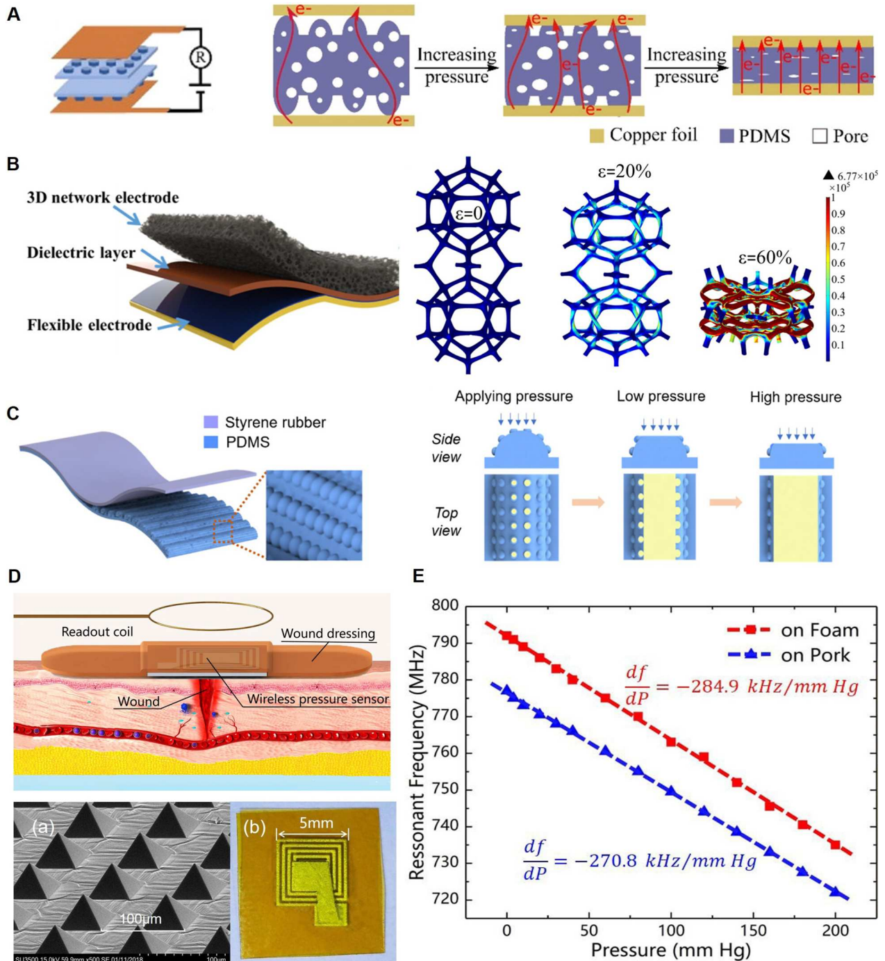
Fig. 3. Schematic illustrating the structure and sensing mechanism of (A) A piezoresistive pressure sensor with PDMS/MWCNTs composites patterned with microstructures [94], (B) A capacitive pressure sensor consisting of MXene nanocomposite dielectric and a 3D network electrode (3DNE) [98], and (C) A triboelectric pressure sensor composed of styrene butadiene rubber (SBR) and patterned poly(dimethylsiloxane) (PDMS) [102]. (D) An LC (inductor-capacitor) pressure sensor consisting of a pyramidal PDMS layer and a spiral inductor for wireless wound monitoring [105]. (E) Measured resonant frequency vs. applied pressure when the LC-sensor-embedded bandage was attached to a pork and a foam, respectively [105].
