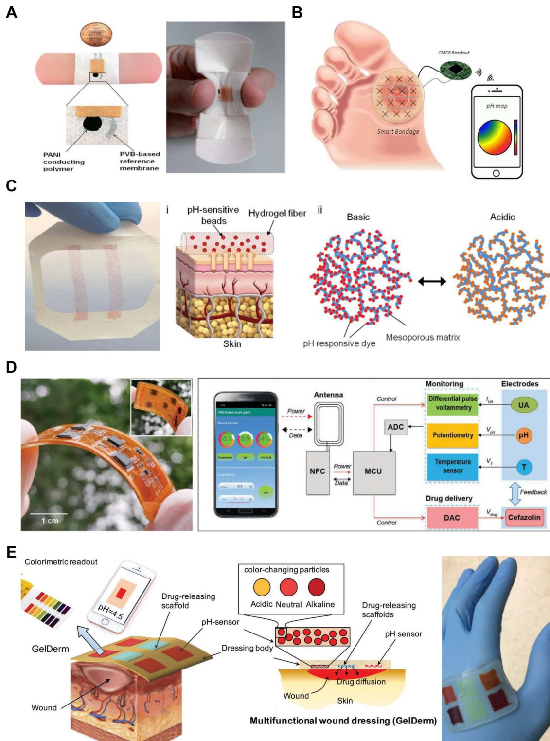
Fig. 5. Wearable pH sensors for wound monitoring. (A) A bandage-like, wearable potentiometric sensor for continuous monitoring of pH. [155] (B) A wireless thread-based pH sensor for monitoring the wound conditions [156]. (C) A flexible pH-responsive hydrogel fiber patch for monitoring epidermal wound conditions [157]. (D) A wearable, wireless wound dressing for online monitoring and on-demand release of antibiotics to wound site [159]. (E) A hydrogel-based multifunctional dressing for colorimetric pH sensing and controlled release of antibiotics [160].
