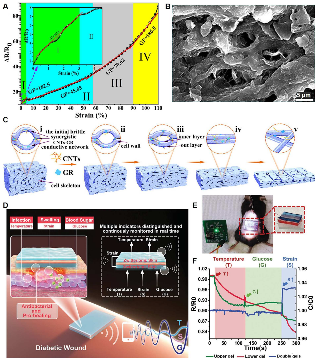
Fig. 4. (A) The sensitivity (gage factor, GF) of a strain sensor in different strain ranges [126]. (B) SEM image showing porous conductive polymer composites with synergistic CNTs-GR conductive networks [126]. (C) Schematic of structure evolution with increasing tensile strains [126]. (D) Schematic illustration of a zwitterionic skin sensor that can continuously and simultaneously monitor the strain, temperature and glucose indicators [138]. (E) Schematic photograph of real-time monitoring on a diabetic mouse wound [138]. (F) Resistance and capacitive response curves in terms of temperature ( T ), glucose concentration ( G ), and strain ( S ) that are continuously monitored and distinguished in real time [138].
