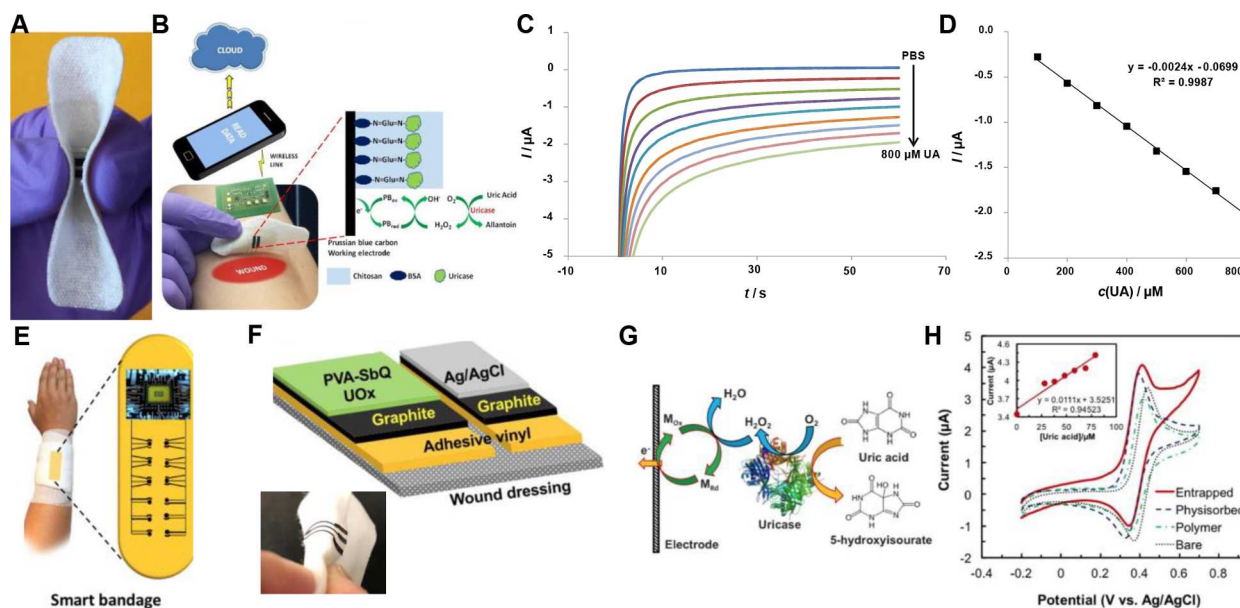
Fig. 6. Wearable uric acid sensors for wound monitoring. (A) Optical image of a wearable enzymatic uric acid sensor. (B) Working principle of the wearable uric acid sensor. (C) The chronoamperograms and (D) linearity of the wearable uric acid sensor over the physiologically relevant concentration from 100 to 800 μM [162]. (E) A wearable enzymatic uric acid sensor for continuous wound monitoring. (F) Schematics for the surface functionalization of working and reference electrodes. (G) Working principle of the enzymatic uric acid sensor. (H) The uricase entrapped electrode shows a superior response towards the detection of uric acid [163].
