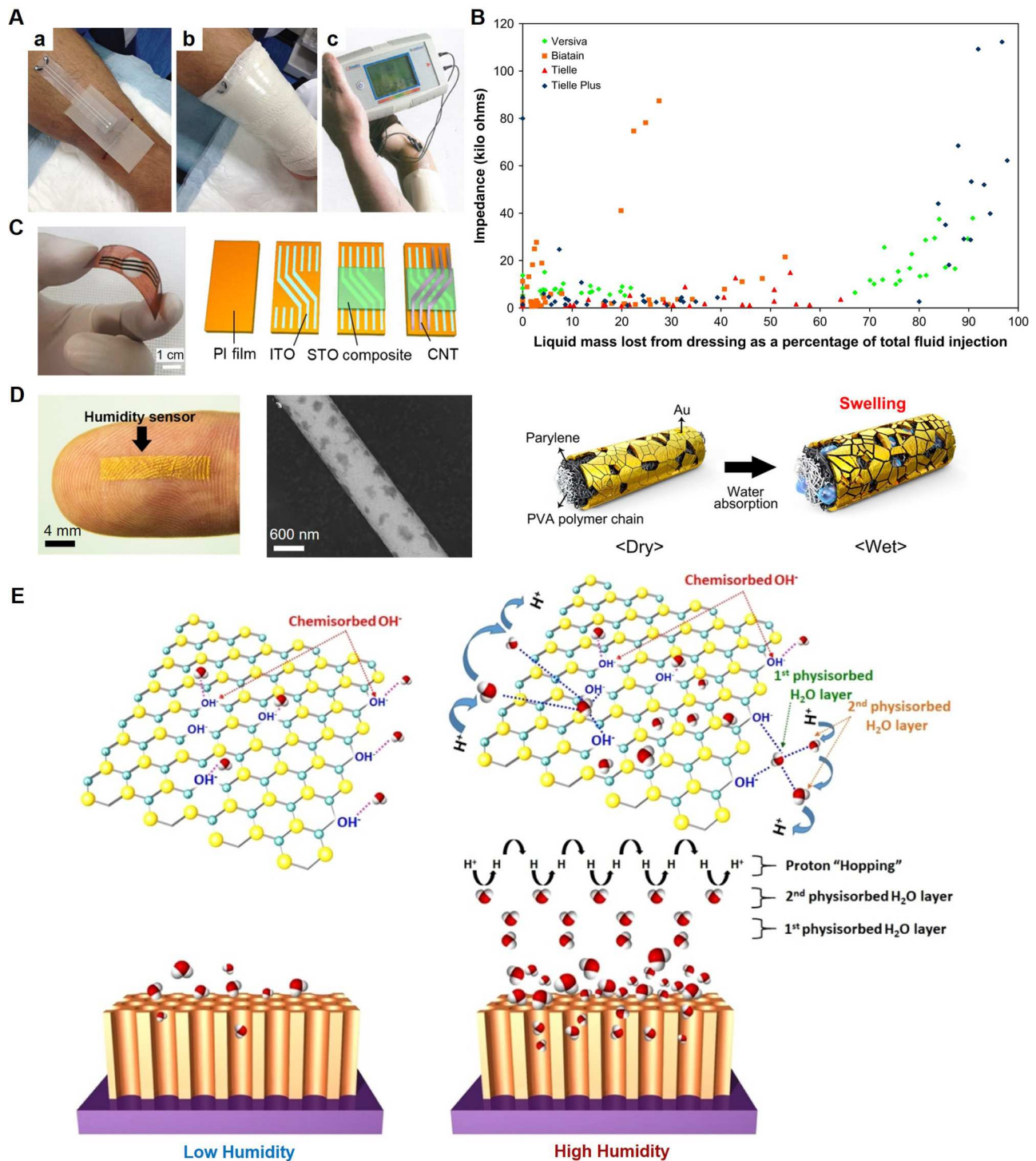
Fig. 2. (A) WoundSense sensor for moisture monitoring in the wound bed: (a) sensor underneath dressing, (b) sensor after dressing, and (c) measurement with a WoundSense meter [64]. (B) Relationship between the percentage of liquid lost from the dressing and the measured impedance via paired silver/silver chloride electrodes embedded in the dressing [63]. (C) Transparent humidity sensors with perovskite-structured SrTiO 3 (STO) composites [73]. (D) A breathable nanomesh humidity sensor composed of parylene C-encapsulated PVA polymer chains and a discrete gold surface [76]. (E) Schematic illustration of the humidity sensing mechanism including the chemisorption of hydroxyl ions (OH - ) at low humidity conditions, and the physisorption of water molecules followed by proton hopping at high humidity conditions [79].
