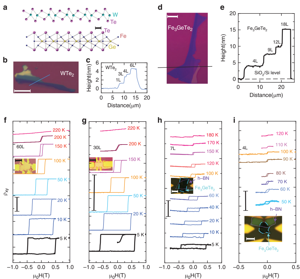
Fig. 1 Thickness characterization and layer-dependent transport properties. a Schematic graph for \text{WTe}_2 on \text{Fe}_3\text{GeTe}_2 . Scale bar: 2 \text{ \AA} . b Microscopic image of exfoliated \text{WTe}_2 flakes. Scale bar: 10 \mu\text{m} . c Cross-sectional profile of the \text{WTe}_2 flakes along the blue line shown in (b) . d Microscopic image of exfoliated \text{Fe}_3\text{GeTe}_2 thin films. Scale bar: 10 \mu\text{m} . e Cross-sectional profile of the \text{Fe}_3\text{GeTe}_2 flakes along the black line shown in (d) . Temperature dependence of Hall resistivity for f 60L, g 30L, h 7L, and i 4L \text{Fe}_3\text{GeTe}_2 flakes showing that the Curie temperature decreases as the thickness of \text{Fe}_3\text{GeTe}_2 decreases. Insets show the devices for the measurements separately and the scale bar in the inset: 10 \mu\text{m} . Resistivity is shifted for clarity. The vertical scale bars are 10 \Omega for (f-h) and 100 \Omega for (i) .
