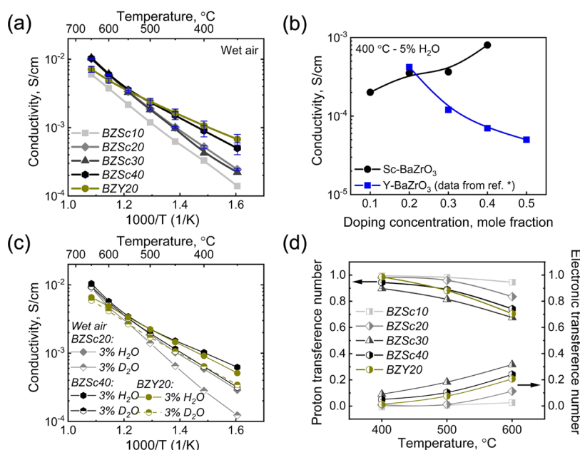
Figure 3. Conductivity and electronic conduction of a series of Sc-doped BaZrO 3 . (a) Total conductivity in 3% H 2 O ( p_{\text{H}_2\text{O}}^* = 0.03 atm)–air. (b) Comparison of total conductivity at 400 °C and 5% H 2 O ( p_{\text{H}_2\text{O}}^* = 0.05 atm)–H 2 of Sc- and Y-doped BaZrO 3 versus doping concentration. * Y-doped BaZrO 3 data reproduced from ref 6. (c) Isotope effect: conductivity of BZSc20, BZSc40, and BZY20 in 3% H 2 O–air and in 3% D 2 O–air. (d) Protonic and electronic transference numbers as a function of temperature for the Sc-doped BaZrO 3 materials and BZY20.
