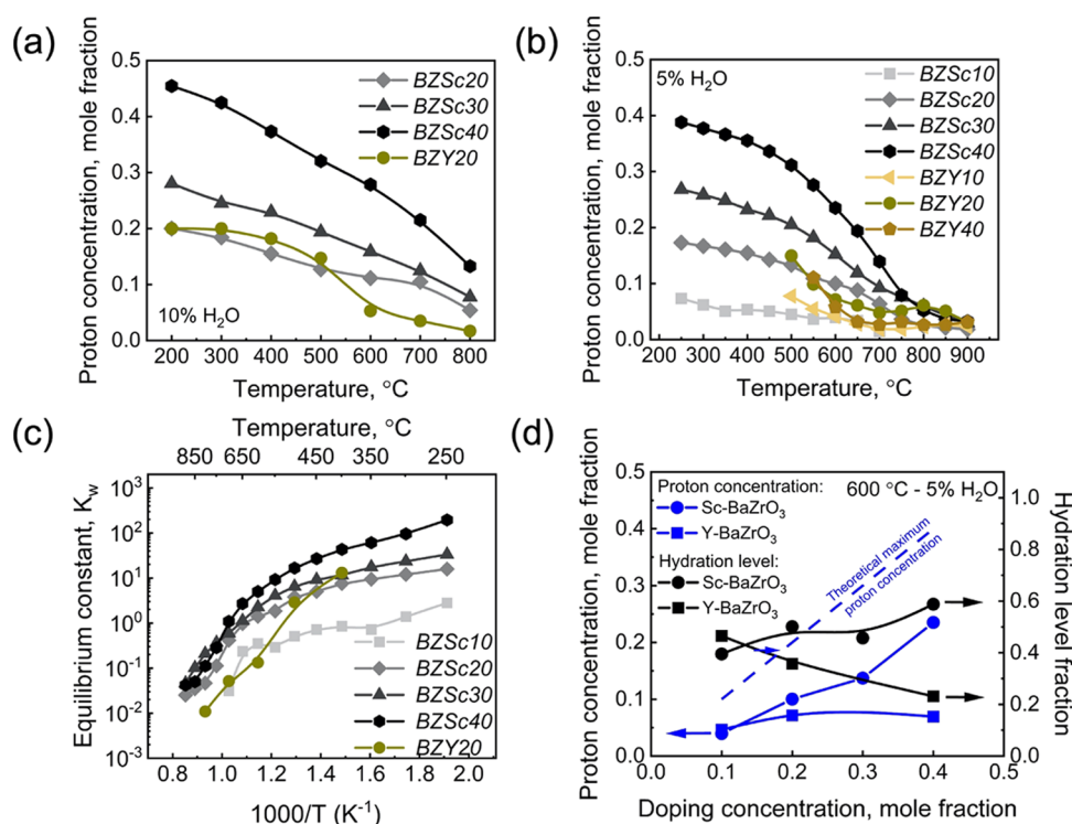
Figure 4. Hydration of Sc-doped and Y-doped BaZrO 3 . (a) Proton concentration as a function of temperature in 10% H 2 O ( p_{\text{H}_2\text{O}}^* = 0.1 atm)–N 2 . (b) Proton concentration as a function of temperature in 5% H 2 O ( p_{\text{H}_2\text{O}}^* = 0.05 atm)–N 2 . (c) Hydration equilibrium constants. (d) Comparison of proton concentration and hydration level (actual proton concentration/theoretical maximum proton concentration) at 600 °C and 5% H 2 O ( p_{\text{H}_2\text{O}}^* = 0.05 atm)–N 2 of Sc- and Y-doped BaZrO 3 versus doping concentration.
