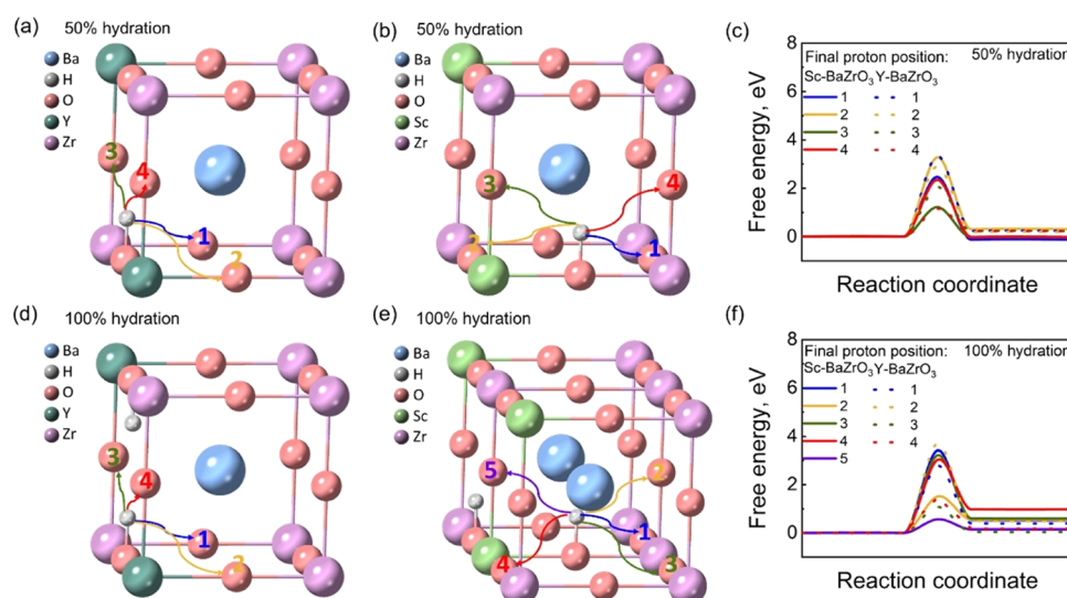
Figure 7. Density functional theory calculation for proton migration of 25 mol % Y- or Sc-doped BaZrO 3 . Proton migration paths in the lattice at 50% of hydration for (a) Y-doped BaZrO 3 and (b) Sc-doped BaZrO 3 . (c) Potential energy profiles for the proton migration paths in panels (a) and (b) for Sc-doped BaZrO 3 and Y-doped BaZrO 3 . Proton migration paths in the lattice at 100% of hydration for (d) Y-doped BaZrO 3 and (e) Sc-doped BaZrO 3 . (f) Potential energy profiles for the proton migration paths in panels (d) and (e) for Sc-doped BaZrO 3 and Y-doped BaZrO 3 .
