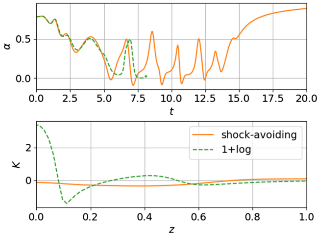
FIG. 2. Comparison of the evolution of a near-critical \ell = 2 Teukolsky wave (with amplitude \mathcal{A} = 0.004955 ) with 1 + \log versus shock-avoiding slicing. In the top panel we show the lapse \alpha at the origin as a function of coordinate time t ; in the bottom panel we show the mean curvature K along the symmetry axis at coordinate time t \simeq 7.83 , shortly before the evolution with 1 + \log slicing crashes. We note that the shock-avoiding slicing condition results in the lapse becoming negative during short intervals of time.
