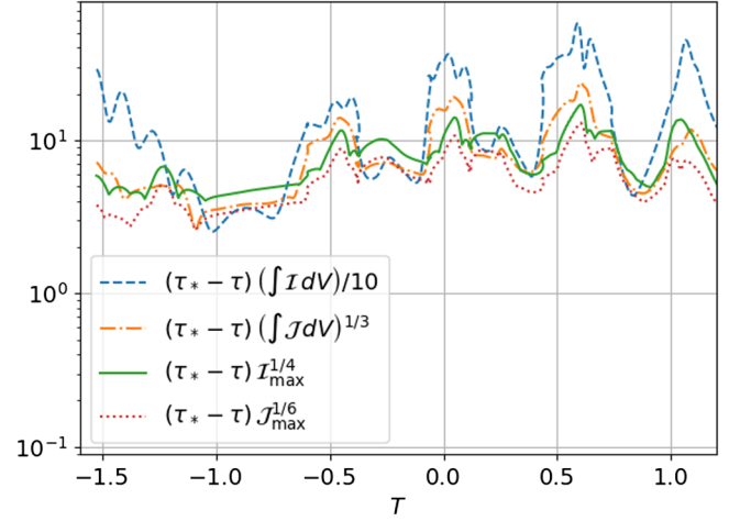
FIG. 4. Curvature measures as a function of slow time T = -\log(\tau_* - \tau) for the near-critical \ell = 2 wave with amplitude \mathcal{A} = 0.00495634 and assuming \tau_* = 4.6 .
