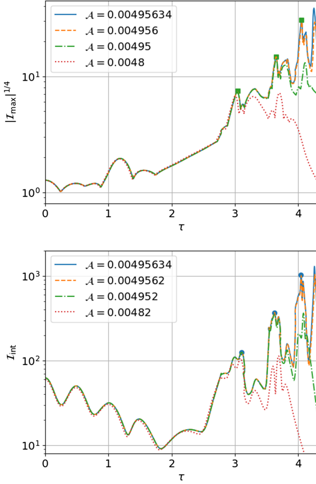
FIG. 3. The maxima (14) (top panel) and integrals (15) (bottom panel) of \mathcal{I} as a function of proper time \tau (as measured at the center) for \ell = 2 waves with different amplitudes \mathcal{A} . In addition to our highest-amplitude subcritical data (for \mathcal{A} = 0.00495634 ) we selected amplitudes \mathcal{A} for which a newly emerging peak in the curvature is approximately as high as the previous peak. The dots and squares mark the times and values of the first three curvature peaks.
