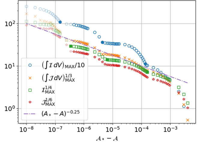
FIG. 9. Global measures of the maximum curvature attained for quadrupolar \ell = 2 waves as a function of amplitude \mathcal{A} , assuming \mathcal{A}_* = 0.00495635 . The filled symbols correspond to the amplitudes shown in Fig. 3 for which a new peak in the curvature emerges and starts dominating over a previous peak; these amplitudes therefore correspond to a “kink” in the scaling plot shown here. Results for near-critical amplitudes, for which we believe that numerical error close to the origin leads to an overestimate in our values of the curvature maxima, are included as shaded symbols only.
