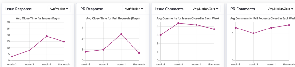
Figure 5: Version 2: Trends. This section of the dashboard displays trends of some useful metrics in the past four weeks to provide maintainers some context of how the project has been doing. This section also displays the logins of new contributors and active contributors with links to their profile pages.
