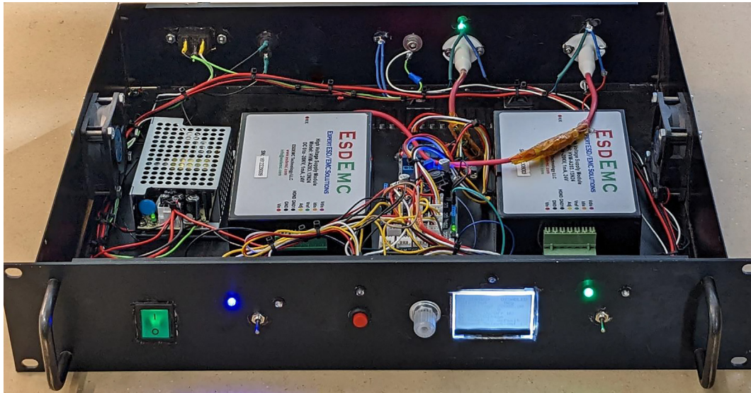
Fig. 1. Assembled HV power supply.
