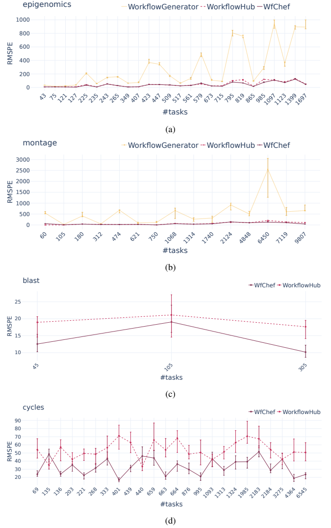
Figure 6: RMSPE of simulated task start dates for Epigenomics (a) and Montage (b), Blast (c) and Cycles (d) workflow instances. Points are average values. Error bars show the range between the third quartile (Q3) and the first quartile (Q1), and minimum and maximum values as black dots.
