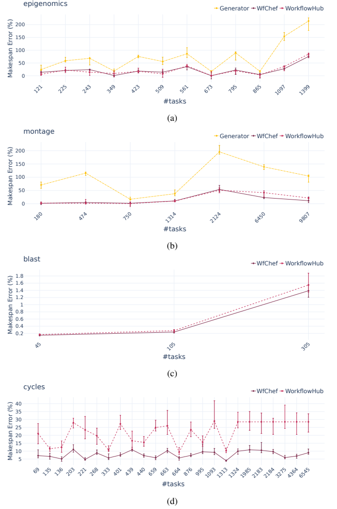
Figure 5: Makespan error for Epigenomics (a), Montage (b), Blast (c), and Cycles (d) workflows instances. Points are average values. Error bars show the range between the third quartile (Q3) and the first quartile (Q1), and minimum and maximum values as black dots.
