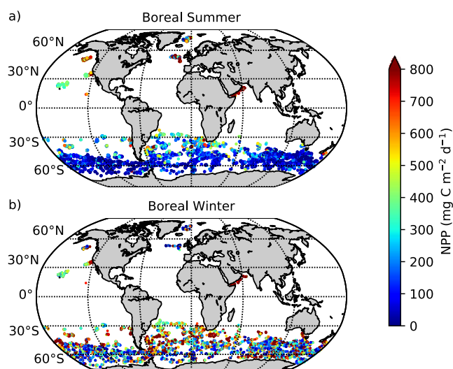
Figure 9. Global patterns in float-based vertically integrated net primary production ( \text{mg C m}^{-2} \text{d}^{-1} ) obtained by the carbon-based productivity model \text{CbPM}_{\text{Argo}} averaged for (a) boreal spring and summer months (April–September) and (b) boreal fall and winter months (October–March).
