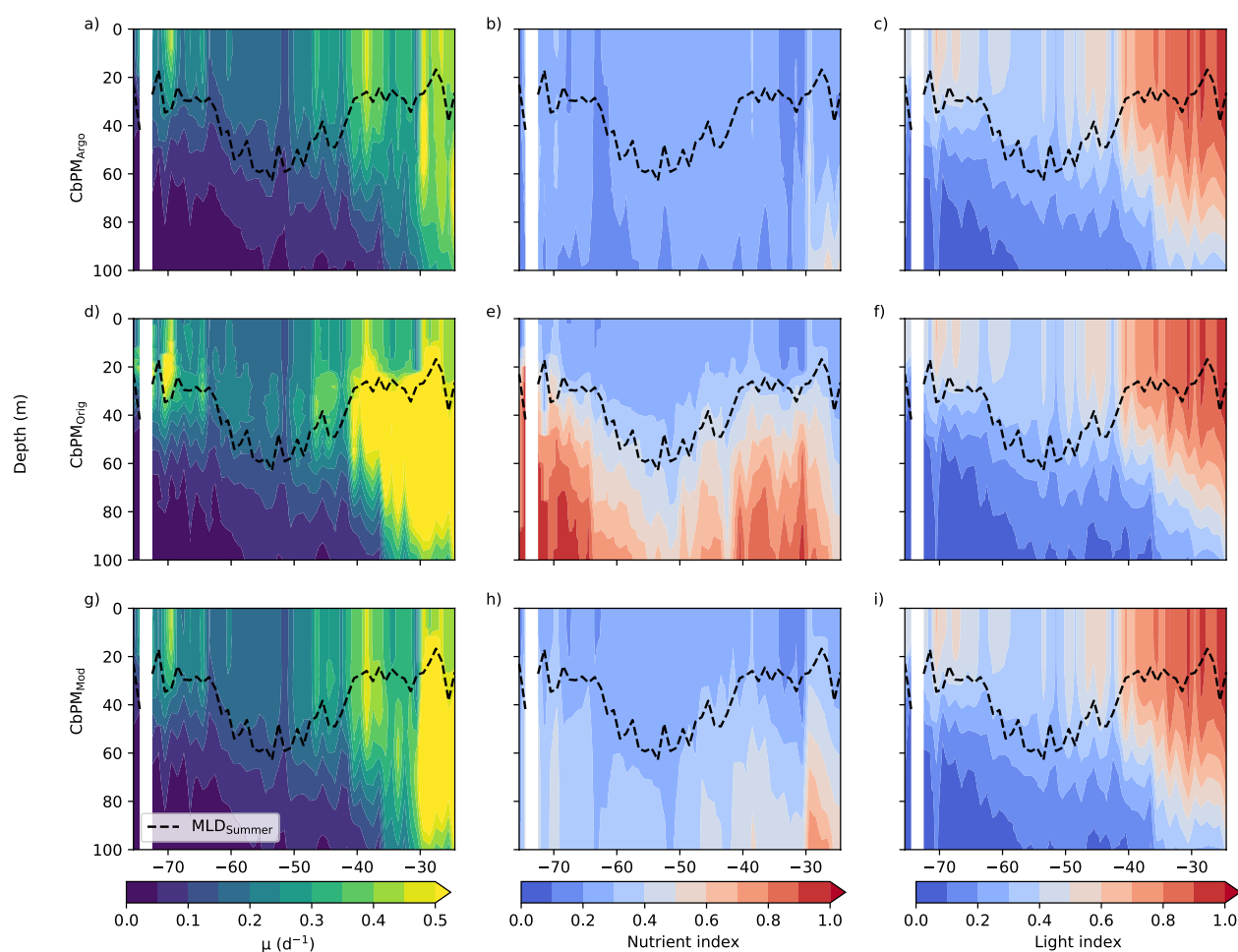
Figure 4. Zonally and seasonally averaged phytoplankton (a) division rate ( \mu , \text{d}^{-1} ), (b) nutrient index (unitless), and (c) light index (unitless) inferred by the carbon-based productivity model ( \text{CbPM}_{\text{Argo}} ). Panels (d–f) show the same variables inferred by the \text{CbPM}_{\text{Orig}} . Panels (g–i) show the same variables inferred by the \text{CbPM}_{\text{Mod}} . All variables were previously binned into a 1^\circ by 1^\circ grid.
