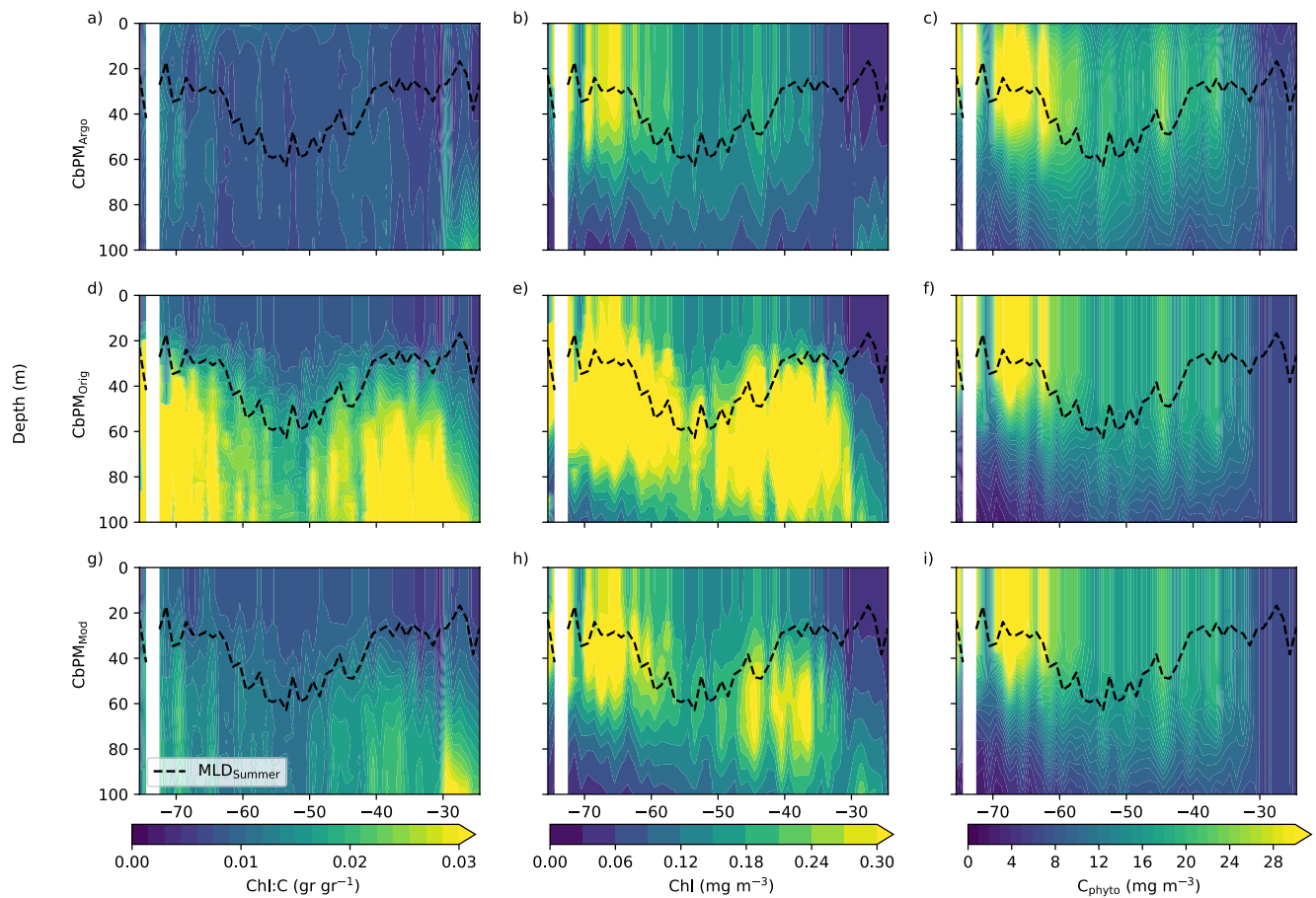
Figure 5. Zonally and seasonally averaged phytoplankton (a) Chl:C ratio ( \text{gr gr}^{-1} ), (b) Chl ( \text{mg m}^{-3} ), and (c) C_{\text{phyto}} ( \text{mg m}^{-3} ) used by the carbon-based productivity model ( \text{CbPM}_{\text{Argo}} ). Panels (d–f) show the same variables inferred by the \text{CbPM}_{\text{Orig}} . Panels (g–i) show the same variables inferred by the \text{CbPM}_{\text{Mod}} . All variables were previously binned into a 1^\circ by 1^\circ grid.
