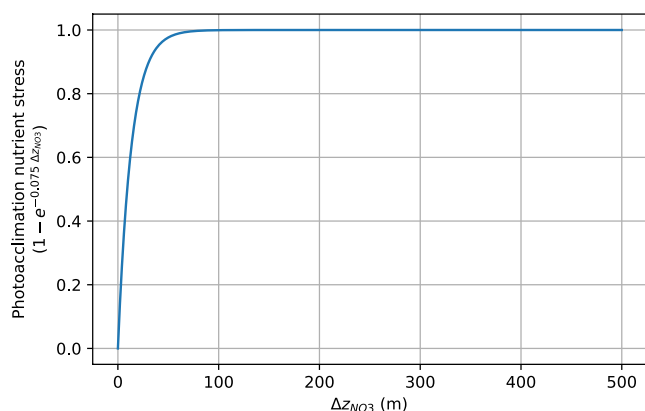
Figure 1. Relationship between the distance separating any given depth below mixed layer depth and the nitracline ( \Delta z_{\text{NO}_3} ) versus the modeled photoacclimation nutrient stress below the mixed layer ( 1 - e^{-0.075 \Delta z_{\text{NO}_3}} ) in the original carbon-based productivity model (Westberry et al., 2008).
