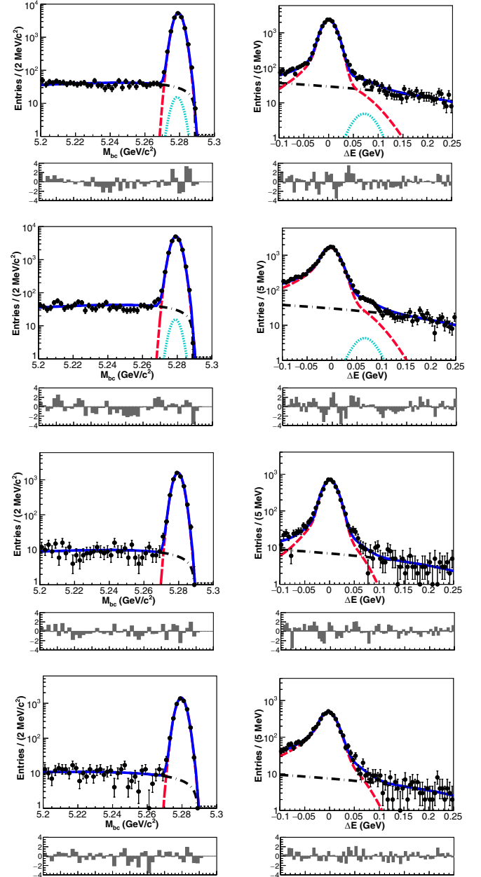
FIG. 1. Left (right) panels: M_{bc} ( \Delta E ) projections of two-dimensional unbinned extended maximum-likelihood fits to the data events that pass the selection criteria for B^+ \rightarrow J/\psi(\mu\mu)K^+ (first row), B^+ \rightarrow J/\psi(ee)K^+ (second row), B^0 \rightarrow J/\psi(\mu\mu)K_S^0 (third row), and B^0 \rightarrow J/\psi(ee)K_S^0 (fourth row) in the log scale. Points with error bars are the data; blue solid curves are the fitted results for the signal-plus-background hypothesis; red dashed curves denote the signal component; black dash-dotted and cyan dotted are combinatorial and [\pi^+J/\psi] backgrounds, respectively. The lower plots show the deviation of data from the fit prediction normalized by the data uncertainty.
