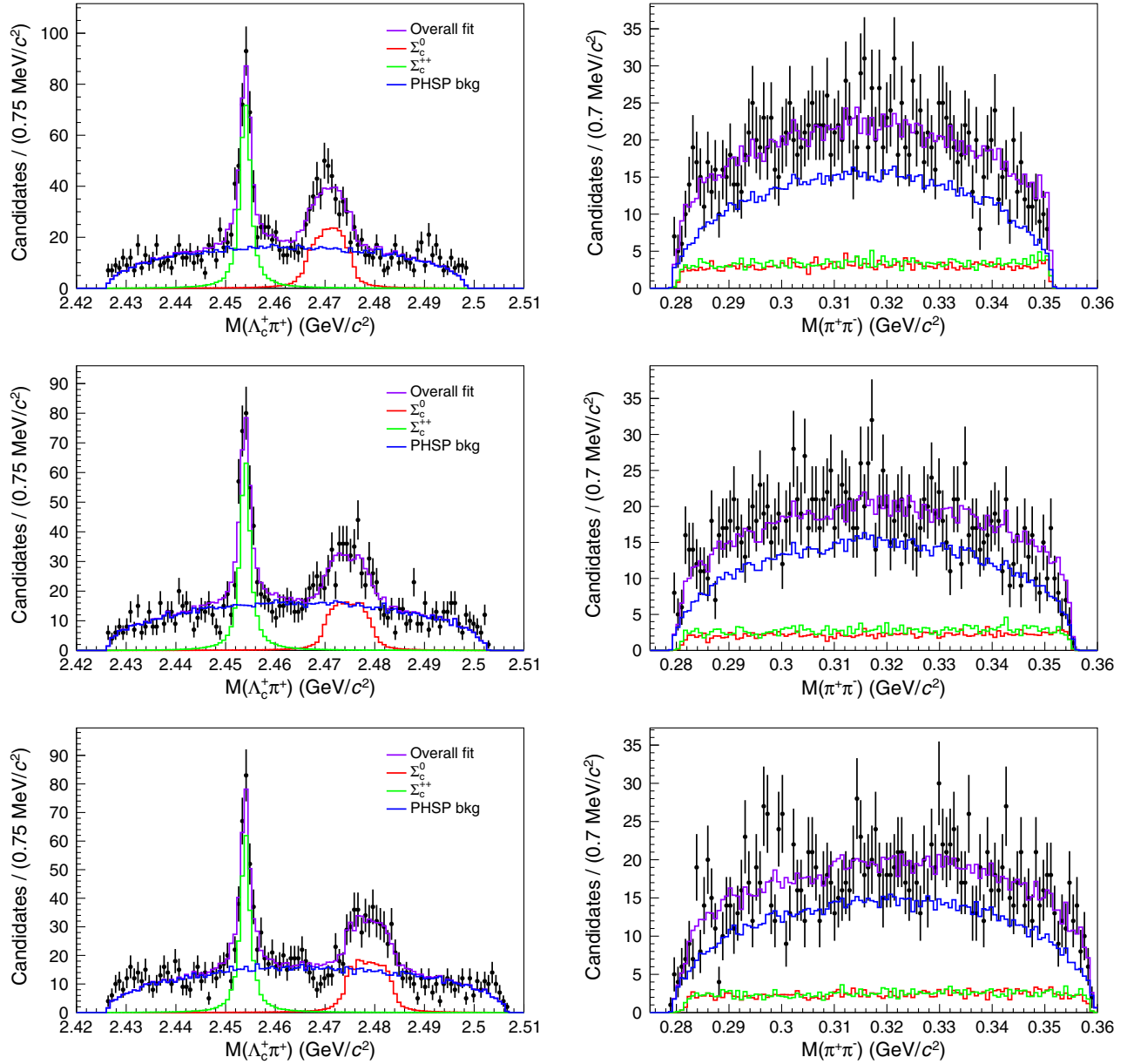
FIG. 6. Projections of the Dalitz plot fits of the three sidebands on the right side of the signal region. The overall fitted distribution and the individual fitted components are shown alongside the experimental data.
