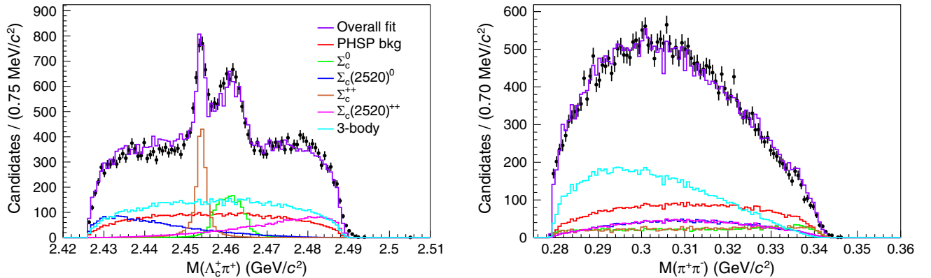
FIG. 3. Dalitz plot fit result plotted as projections. Solid lines show the overall fitted distribution and its individual components as indicated in the legend. PHSP refers to “phase space”. More explanations in the text.
