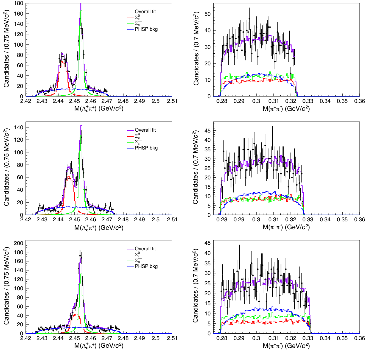
FIG. 5. Projections of the Dalitz plot fits of the three sidebands on the left side of the signal region. The overall fitted distribution and the individual fitted components are shown alongside the experimental data.
