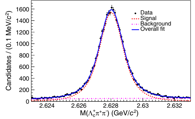
FIG. 1. Distribution of the invariant mass M(\Lambda_c^+\pi^+\pi^-) where the \Lambda_c^+ mass is fixed to the PDG value. The solid line shows the overall distribution and the dashed lines show the individual signal and background components.
