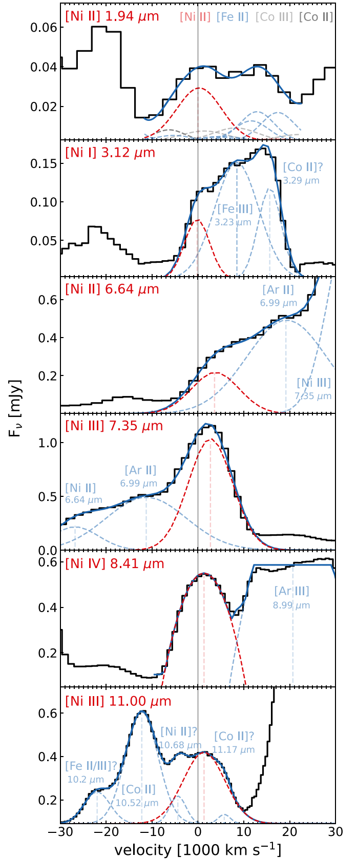
Figure 10. Observed NIR and MIR nickel emission-line profiles for SN 2021aefx at +255 days (black) compared to model line emission from Gaussian distributions, except for [Ni IV] 8.405 \mu\text{m} , which is better fit by emission from a uniform spherical emission distribution. The model profile for the central line is shown in dashed red, with contributions from other lines shown in dashed blue and the full modeled superposition of lines shown in solid blue.
