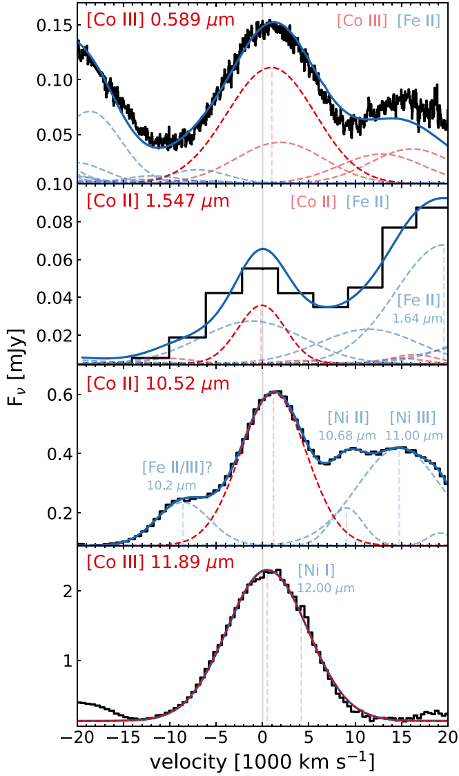
Figure 9. Cobalt emission-line profiles of SN 2021aefx at +255 days (black) across the optical, NIR, and MIR compared with model line emission from Gaussian distributions of emission. The model profile for the central line is shown in dashed red, with contributions from other lines shown in dashed blue and the full modeled superposition of lines shown in solid blue.
