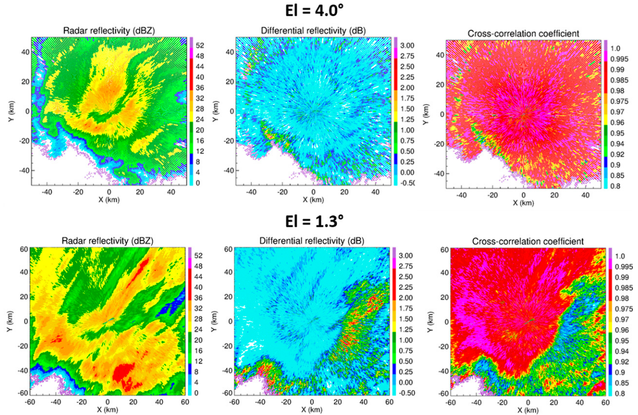
FIG. 3. PPIs of Z , Z_{DR} , and CC at (top) EI = 4.0^\circ and (bottom) EI = 1.3^\circ for the storm on 5 Feb 2020 in Oklahoma observed by the KTLX WSR-88D at 1105 UTC.
