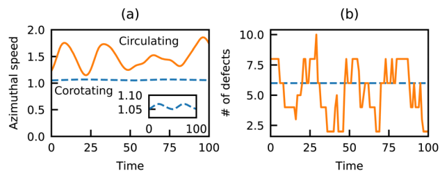
Fig. 5 Distinction between the corotating and the circulating states. (a) Average azimuthal speed ( \vec{u} \cdot \hat{\theta} ) as a function of time for a representative corotating state (blue dashed line, R_i = 6 , W = 6 ) and a circulating state (orange continuous line, R_i = 1 , W = 10 ). While both have a steady circulation on average, there is significant variation in the instantaneous flow of the circulating state, as opposed to the weakly sinusoidal variation in the corotating state (the inset shows a zoomed-in plot of the same). (b) Total number of defects as a function of time for the same two datasets. The number of defects remains constant for the corotating case, whereas it fluctuates for the circulating case, indicating annihilation and proliferation.
