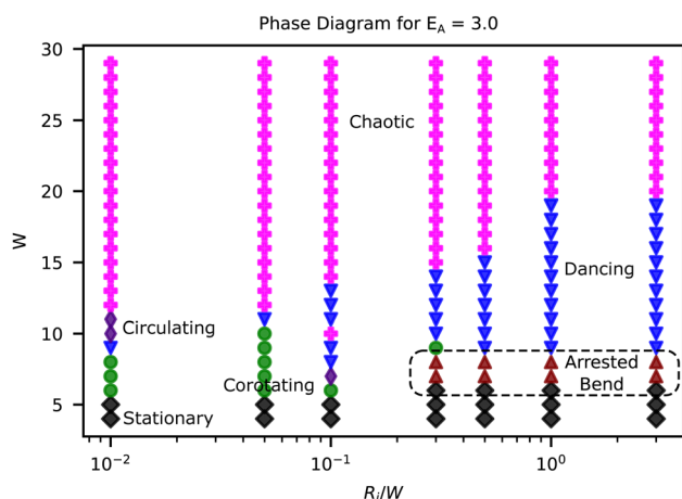
Fig. 7 Phase diagram for strong anchoring conditions (with E_A = 3.0 ). The markers correspond to the same states as in Fig. 3: (i) stationary state (grey diamonds), (ii) corotating state (green circles), (iii) circulating state (indigo thin diamonds), (iv) dancing state (blue triangles), and (v) chaotic state (magenta pluses), except for the maroon upward triangles that indicate the arrested bend instability state. This phase diagram reveals the absence of the corotating state (green circles) for high anchoring and low curvature.
