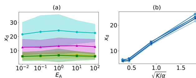
Fig. 10 Alignment decay length x_d as a function of activity and anchoring strength. Plots of x_d (defined in Fig. 9) as a function of (a) anchoring strength and (b) the active length scale, analogous to Fig. 9(c) and (d), indicating that x_d is independent of the anchoring strength. The legend used in (a) and (b) is identical to that of Fig. 9(c) and (d) respectively.
