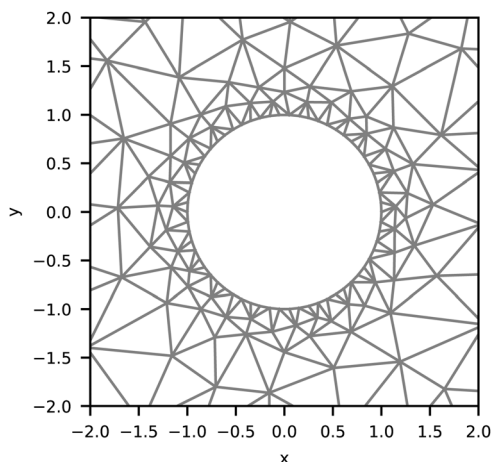
Fig. 11 Close up of the finite-element mesh for R_i = 1 , W = 5 . The mshr library automatically generates smaller elements near the inner radius.
