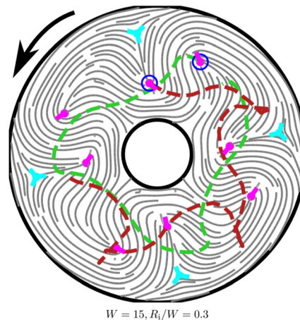
Fig. 6 Curvature-induced drift in the dancing state for W = 15 and R_i/W = 0.3 . In this case, due to the asymmetry of the inner and outer curvature, the flow acquires a drift (see Movie S6, ESI†) despite there being an equal number of defects moving in each direction. The dotted green line highlights the trajectory of a defect moving uninterruptedly anti-clockwise, while the red dotted line highlights the trajectory of a defect moving clockwise, undergoing annihilation and nucleation periodically at the outer edge. This asymmetry of defect motions creates a net flow in the counter-clockwise direction.
