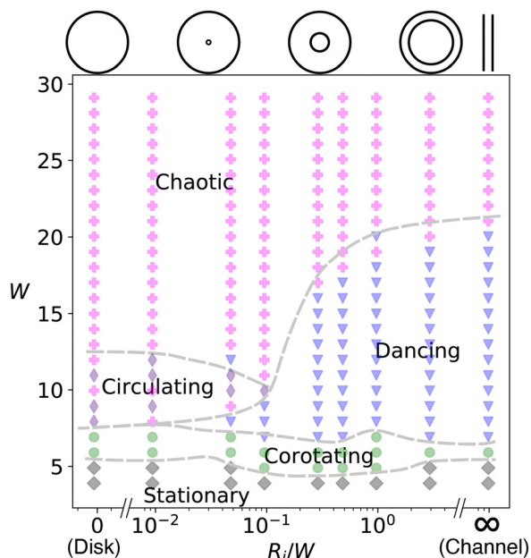
Fig. 3 Shape-size phase diagram for active nematics in annuli. Steady states as a function of width W and the ratio of the inner radius to width R_i/W : (i) Stationary state (meaning \partial_t \vec{Q} = 0 = \partial_t \vec{u} , grey diamonds), (ii) Corotating state (green circles), (iii) Circulating state (indigo thin diamonds), (iv) Dancing state (blue triangles), and (v) Chaotic state (magenta pluses). The indicated shapes for various R_i/W on the top are a guide to the eye and not to scale. R_i/W = 0 corresponds to a disk of radius W , whereas R_i/W = \infty corresponds nominally to a channel simulation with width W , length 20W , and periodic boundary conditions at the channel ends. For these simulations, we apply a no-slip boundary condition for the velocity, and weak parallel anchoring for the director, with E_A = 0.01 . The dashed grey lines are drawn manually as a guide to identify the approximate boundaries between different steady-state behaviors.
