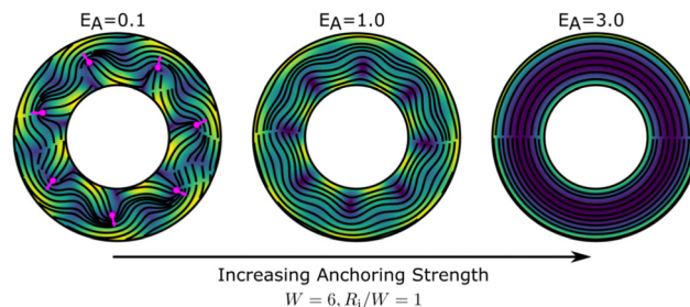
Fig. 8 The corotating state disappears at high anchoring strengths. Snapshots of the steady state for W = 6 , R_i/W = 1 for different anchoring strengths. (left) For low anchoring strengths, the -\frac{1}{2} defects are easier to form and we observe the corotating state. (middle) For intermediate anchoring, the bend instability is arrested. (right) For high anchoring strengths, the bend instability is completely suppressed. The width for the onset of the dancing state remains independent of anchoring strength. The color represents the scalar order parameter S with the same color-map as in Fig. 1.
