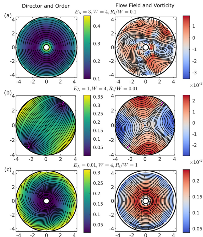
Fig. 4 Various stationary states ( \partial_t \vec{Q} = 0 = \partial_t \vec{u} ) of active nematics observed in disk-like annuli. The left panel shows the director field with streamlines and the scalar order parameter S with the color. The right panel shows the corresponding flow field, also shown as directed streamlines and the vorticity |\nabla \times \vec{u}| with the color. (a) State with \vec{u} \sim 0 ( |\nabla \times \vec{u}| \sim 10^{-3} ) and the director in a +1 defect configuration. Here, E_A = 3 , W = 4 , R_i/W = 0.1 . (b) Dipolar state with two defects and \vec{u} \sim 0 ( |\nabla \times \vec{u}| \sim 10^{-3} ), as also observed in disks in ref. 59. Here, E_A = 1 , W = 4 , R_i/W = 0.01 . (c) For low anchoring strength, we can observe a spiral configuration of the nematic, with a non-zero but constant velocity ( \vec{u} \neq 0 , \partial_t \vec{u} = 0 ). Here, E_A = 0.01 , W = 4 , R_i/W = 0.1 .
