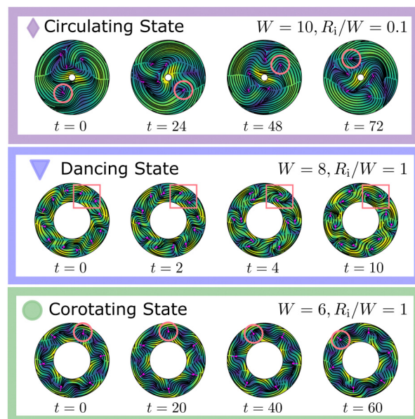
Fig. 2 Dynamical steady states in active nematics confined to annulus geometries. (top) The circulating state, as observed for W = 10 and R_i/W = 0.1 . A single defect going around the channel is shown with a red circle to highlight the circulation. (middle) The dancing state, as observed for W = 8 and R_i/W = 1 . The highlighted region shows the dancing behavior of a defect pair over time. (bottom) The corotating state, as observed for W = 6 and R_i/W = 1 . The highlighted defect shows the corotating motion of the train of defects. The symbols correspond to those used to identify these states in the phase diagram in Fig. 3. The color represents the scalar order parameter S with the same color-map as in Fig. 1. All times start at an arbitrary point and are in the units of 0.1 simulation times.
