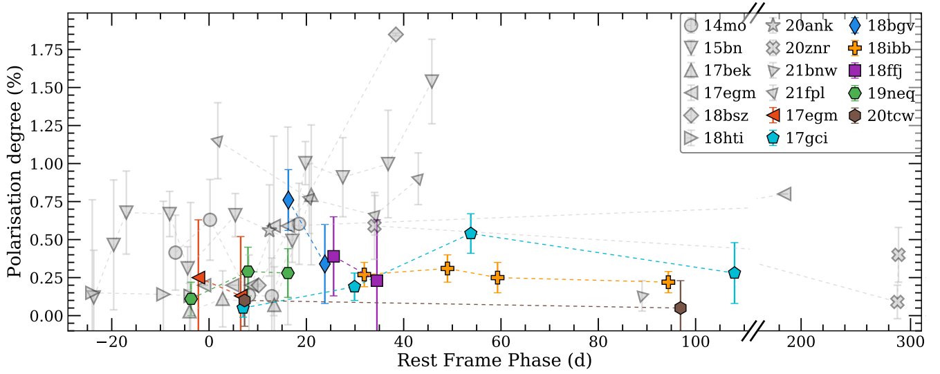
Fig. 4. Polarisation degree vs. rest-frame phase measured from the peak brightness in r/V band. The literature data collected from sources listed in Table 1 are shown with grey markers. The data are in V band (or comparable), apart from SN 2020znr ( R ). No ISP correction is performed for SN 2018bgv. For SN 2018hti, we performed the ISP correction based on values presented in Lee (2019) and for SN 2018bsz we assume the Case A ISP as presented by Pursiainen et al. (2022). We note the break and scale change in the x -axis at 150 d.
