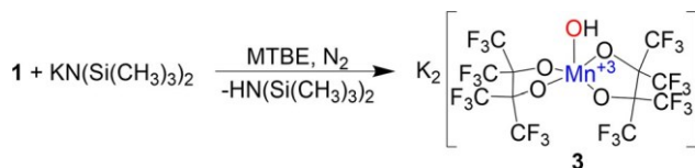
Scheme 3 Synthesis of 3.
