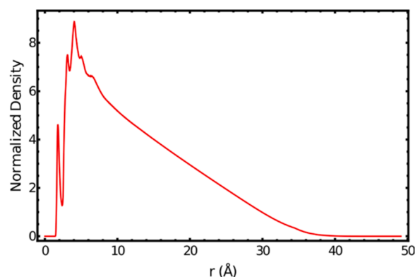
Fig. 5. Normalized \text{SO}_3^- \text{H}_2\text{O} radial density function within a w_0 = 20 AOT RM without any added KCl.
