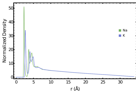
Fig. 6. Normalized SO 3 − - Na + (green line) and SO 3 − - K + (purple line) radial density functions within a w_0 = 20 AOT RM doped with 1.0 M KCl.
