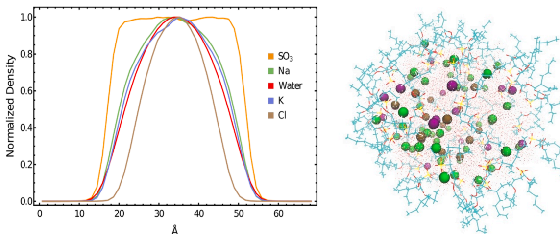
Fig. 4. Normalized density profiles for \text{SO}_3^- (orange line), \text{Na}^+ (green line), \text{H}_2\text{O} (red line), \text{K}^+ (purple line), and \text{Cl}^- (brown line) within a w_0 = 20 AOT RM doped with 1.0 M KCl. The distance on the X-axis is the simulation box length. On the right, a snapshot of the reverse micelle is shown without the isoctane solvent. The water molecules are represented by red dots, sodium ions by green beads, potassium ions by purple beads and chloride ions with brown beads.
