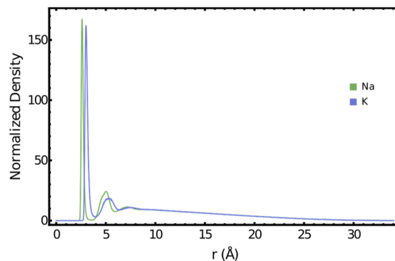
Fig. 8. Normalized Na^+ - Cl^- (green line) and K^+ - Cl^- (purple line) radial density functions within a w_0 = 20 AOT RM doped with 1.0 M KCl.
