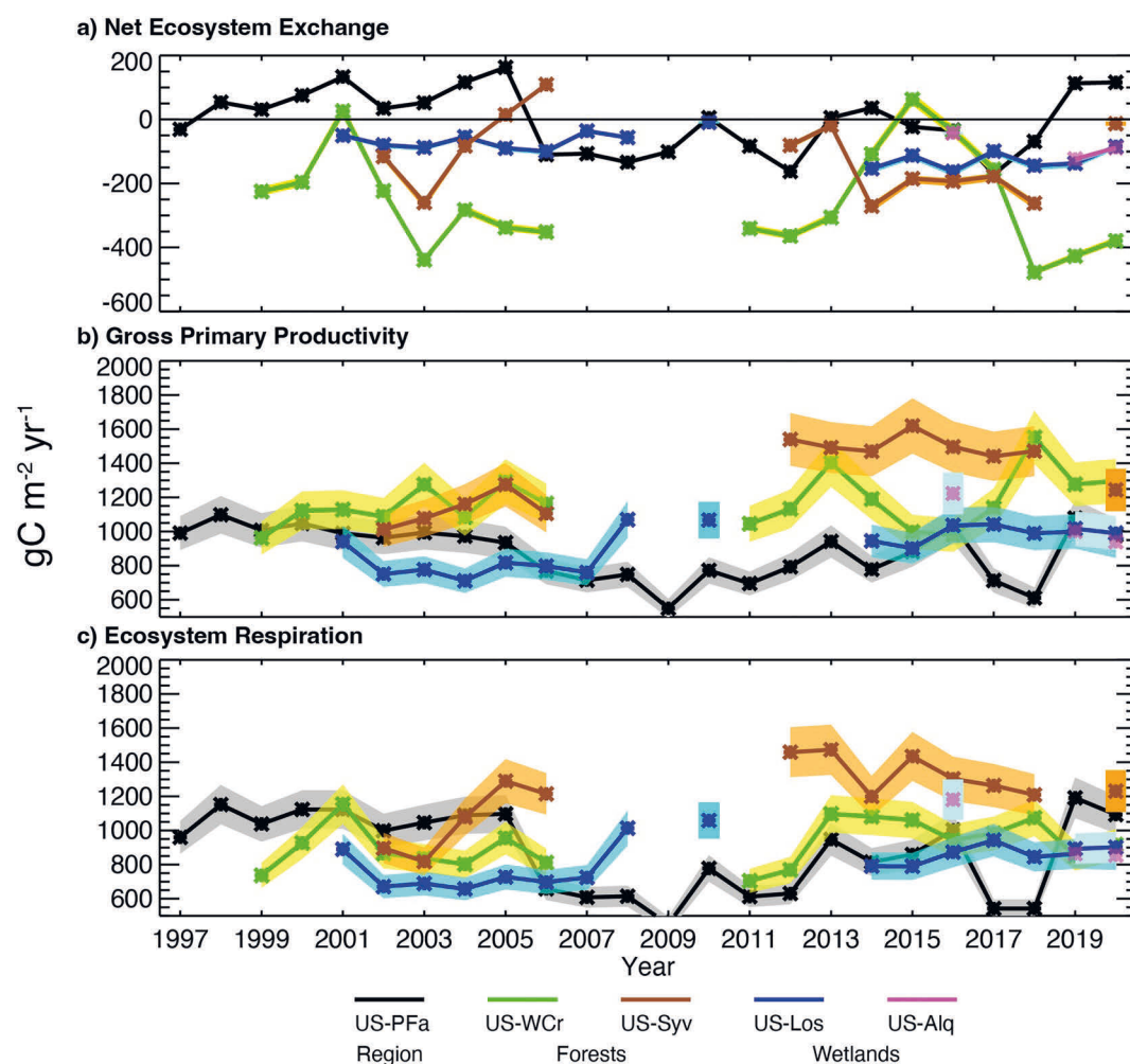
Figure 4. Annual gap-filled total (a) net ecosystem exchange and partitioned (b) gross primary productivity and (c) ecosystem respiration for the regional (US-PFa, black), forests (US-WCr and US-Syv) and wetlands (US-Los and US-ALQ) from 1997 to 2020. Estimated uncertainty shown in shading for each.
