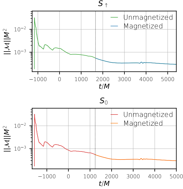
FIG. 23. Evolution of the L_2 norm of the momentum constraint violations for both configurations, with the magnetized disk evolutions overlayed on the nonmagnetized evolutions.
