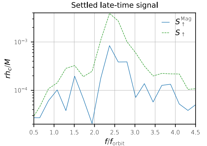
FIG. 18. Characteristic strain for the spinning BH case, for the GW signal emitted during the period when the disk has entered a settled steady state. The solid line is the magnetized case; the dashed shows the signal for an equivalent period in the nonmagnetized case.
