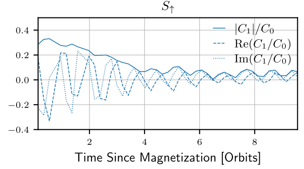
FIG. 8. Amplitude of the normalized m = 1 density mode after magnetic field insertion for the spin-up case. Note that the components of the m = 1 nonaxisymmetric mode take on a slightly nonzero average value at late times in this case. This seems to be due to slight eccentricity that develops due to the nonaxisymmetric variations in accretion that occur intermittently as a result of both the disk nonaxisymmetry and the non-axisymmetry of the seed magnetic field. Our diagnostic measures just the angular m = 1 mode, it does not account for radial distribution of matter and bears no relation to the disk center of mass moment. There is therefore no reason to expect it to always oscillate around zero, and this detail can be ignored as irrelevant to the dynamics of interest.
