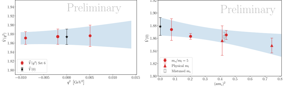
Figure 5: Left: fit of the J/\psi \rightarrow \gamma\eta_c V(q^2) data (red circles) from set 6, with interpolation to q^2 = 0 shown by the black star. Right: chiral-continuum fit of the interpolated (i.e. q^2 = 0 ) data. The grey square shows \hat{V}(0) from the deliberately mistuned m_c (set 3A), but it is not included in this preliminary fit. The red circles are the lattice data on sets 2-6 (excluding 3A), and the black star is the result in the continuum.
