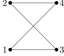
Figure 20: The kernel S(x_1, x_2, x_3, x_4) in pictorial form.
