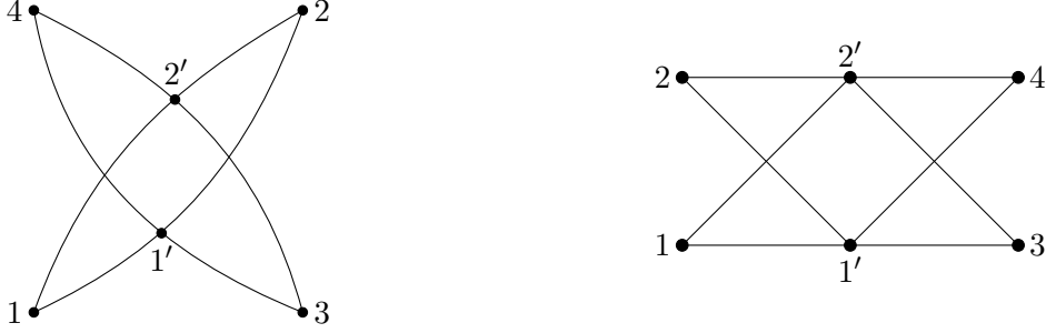
Figure 19: On the left, a diagram showing an event shape for \mathbf{L}[\phi^2]\mathbf{L}[\phi^2] , embedded inside the four-point correlator \langle\phi^2\phi^2\phi^2\phi^2\rangle . We imagine \phi^2(x_1)\phi^2(x_2) creating the detector \mathbf{L}[\phi^2]\mathbf{L}[\phi^2] via the mechanism in figure 18. This detector is then measured in states created by \phi^2(x_3) and \phi^2(x_4) . On the right, we re-draw the same diagram in a simpler way that makes clear that it is the square of the kernel S , which is one of the terms inside SG_{\text{tree}} in equation (5.55).
