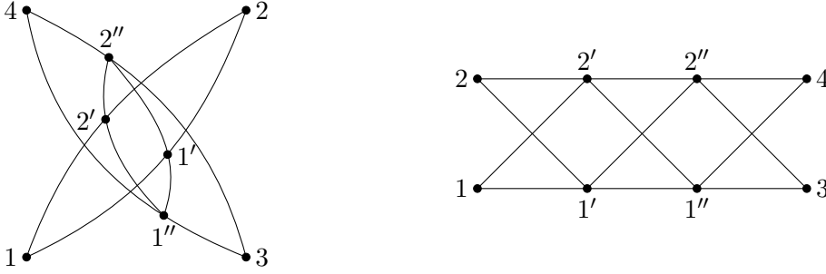
Figure 21: On the left, an embedding of the anomalous dimension diagram from figure 17a inside the four-point correlator \langle \phi^2 \phi^2 \phi^2 \phi^2 \rangle . We imagine \phi^2(x_1)\phi^2(x_2) creating the detector \mathbf{L}[\phi^2]\mathbf{L}[\phi^2] via the mechanism in figure 18. This detector is measured by particles that propagate from x_3, x_4 , split at x'_1 and x'_2 , and are finally detected at x'_1 and x'_2 . On the right, we re-draw the same diagram in a simpler way that makes clear that it is the cube of the kernel S , which is one of the terms inside S^2 G_{\text{tree}} in equation (5.55).
