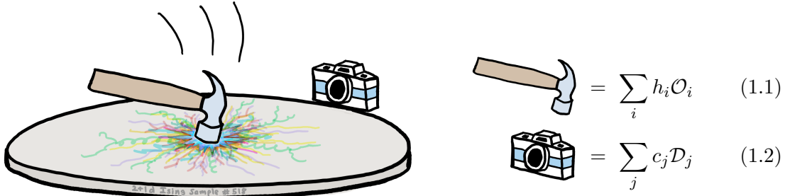
Figure 2: In an experiment involving a QFT \mathcal{Q} , the probe (hammer) can be expanded in operators \mathcal{O}_i that are intrinsic to \mathcal{Q} , schematically eq. (1.1). Similarly, a far-away measurement apparatus (camera) can be expanded in detectors \mathcal{D}_i that are intrinsic to \mathcal{Q} , eq. (1.2). These twin expansions cleanly separate the details of the experiment (contained in the coefficients h_i and c_j ) from the dynamics of the theory (encoded in matrix elements \langle \mathcal{O}_i | \mathcal{D}_j | \mathcal{O}_k \rangle ).
