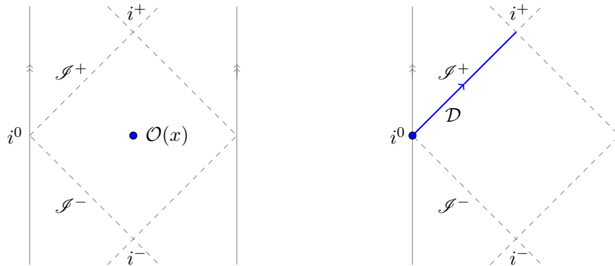
Figure 10: Illustrations of the traditional conformal frame (left), with a local operator \mathcal{O} at a generic point inside Minkowski space, and the detector frame (right), where a detector \mathcal{D} lies along future null infinity \mathcal{I}^+ . The detector \mathcal{D} transforms like a primary operator at spatial infinity i^0 (the blue point), which means that it is invariant under Minkowski translation generators, and this statement is exact in perturbation theory. In a CFT, future null infinity is not a special place, and can be reached by a simple shift on the Lorentzian cylinder. For simplicity of illustration, both figures show the 2d Lorentzian cylinder. For example, in the left figure, the two solid grey lines should be identified. Minkowski space is the interior of the diamond formed by dashed grey lines. The same is true for the figure on the right.
