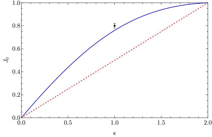
Figure 7: Solid, blue: the \text{Padé}_{3,3} approximant to the intercept J_0(\epsilon) imposing the small- \epsilon expansion (2.29) and known value in d = 2 ( J_0(2) = 1 ). Dashed, red: the formal intercept value for free theory. The data point at \epsilon = 1 is the result from [40], taken with the (non-rigorous) error bar estimated from their figure 12.
