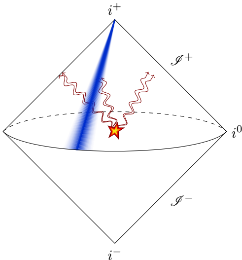
Figure 1: A detector (blue) is a translationally-invariant operator localized at future null infinity \mathcal{J}^+ , capable of measuring properties of a state at late times. Some detectors, such as the average null energy operator \mathcal{E}_2(\vec{n}) , are localized on a light-ray. Other detectors can measure nontrivial angular distributions on the celestial sphere, as indicated by “fuzziness” in the angular directions in the figure.
