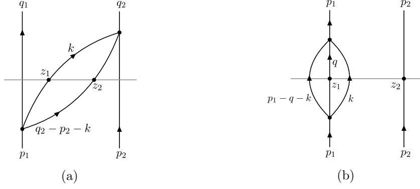
Figure 17: Loop-level contributions to the mixing of \mathcal{H}(z_1, z_2) . (a) Connected diagram which induces “smearing” on celestial sphere. (b) Disconnected diagram for the correction to an individual detector. There exist other diagrams at O(\lambda) and O(\lambda^2) but they do not contain IR divergences.
