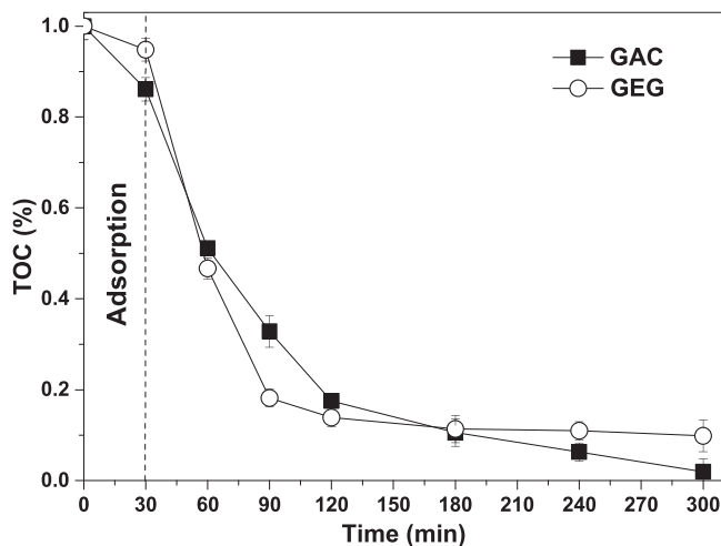
Fig. 8. Performance of the DCF electro-oxidation using two APB reactors in series with GAC and GEG materials. Operational conditions: 5 h, 20% DCF saturation on GAC and GEG, 20 mA cm -2 , 0.1 M Na 2 SO 4 , 25 °C, 1.4 g GAC per cell, 0.6 g GEG per cell, 125 mg DCF L -1 , 64 mg TOC L -1 TOC as initial concentrations.
