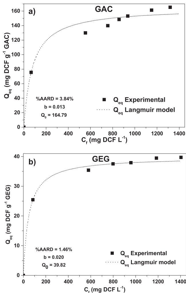
Fig. 4. Experimental DCF adsorption isotherms and Langmuir model ( Q_E = bQ_0C_f / (1 + bC_f) ) fitting for: a) GAC and b) GEG. Experimental conditions: 100–1400 mg DCF L -1 (initial concentration), 0.1 g GAC or 0.2 g GEG, 8 h, 24 °C, and 250 rpm.
