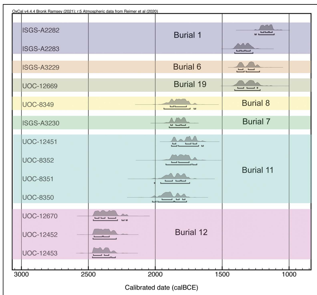
Figure 4. Probability density distributions of calibrated radiocarbon assays from MARP-79 (figure by the authors).
