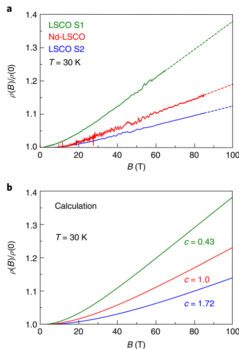
Fig. 3 | Effect of disorder. a , Measured MR at T = 30 K, for Nd-LSCO (red), LSCO S1 (green) and LSCO S2 (blue). The dashed lines are linear extensions of the data. b , Calculated MR at T = 30 K, for three levels of disorder, obtained by setting the prefactor of the elastic scattering term in equation (1) to c = 1.0 (red), 0.43 (green) and 1.72 (blue). The values of c correspond to the variation in the measured \rho_0 values of our three samples (Fig. 1b).
