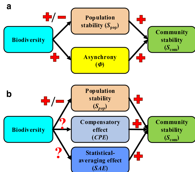
Fig. 1 | Diagram illustrating how biodiversity influences community stability via its effects on species-averaged population stability and species asynchrony. Empirical studies show that biodiversity may increase or decrease population stability, but it generally promotes asynchrony (a; adapted from Xu et al. 7 ). Asynchrony can be further decomposed multiplicatively into an effect of compensatory dynamics (CPE) and a statistical-averaging effect (SAE; b). We assessed how biodiversity separately alters CPE and SAE.
