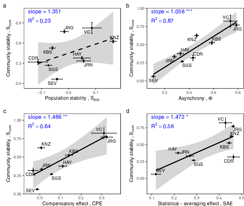
Fig. 3 | Relationships between community stability and its components across the nine sites in the plant survey dataset. The components include: a population stability ( p = 0.187 ), b asynchrony ( p < 0.001 ), c the compensatory effect ( p = 0.009 ), and d the statistical-averaging effect ( p = 0.017 ) across the nine sites in
