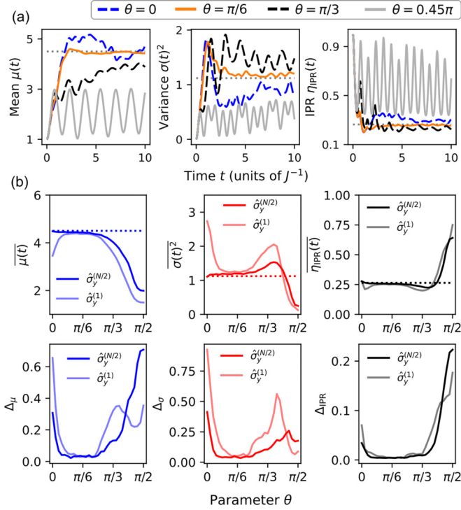
FIG. 3. Measures of the probability distribution \{P_k\} for the tilted-field Ising model with N = 6 and B/J = 1 . (a) Mean \mu(t) , variance \sigma^2(t) , and IPR \eta_{\text{IPR}}(t) of the operator distribution shown as a function of time for the four values of \theta displayed in Fig. 2. Dotted lines correspond to the predictions for Haar-random evolution shown in Table I. Results shown here correspond to \hat{O}(0) = \hat{\sigma}_y^{(N/2)}/\sqrt{2} . (b) Long-time properties of the aforementioned measures, as calculated by the time-averaged value [cf. Eq. (20)] and the time-averaged temporal fluctuations [cf. Eq. (21)]. Plots are shown as a function of the parameter \theta of the Ising model and for choices of the initial operator on the middle site (dark lines) and at the edge (light lines) of the chain.
