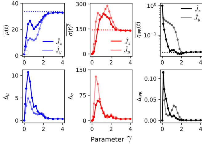
FIG. 6. Shown in the top row are the long-time averages [cf. Eq. (20)] and in the bottom row the averaged temporal fluctuations [cf. Eq. (21)] for the mean, variance, and IPR of the operator distribution for the QKT. Results are shown for N = 2J = 49 , using parameter values for \{\alpha_i, \gamma\} identical to those in Fig. 4, and for two distinct initial operators \hat{O}(0) = \hat{J}_z (dark lines in all plots) and \hat{O}(0) = \hat{J}_y (light lines). All dashed lines correspond to the predictions for Haar-random evolution shown in Table I.
