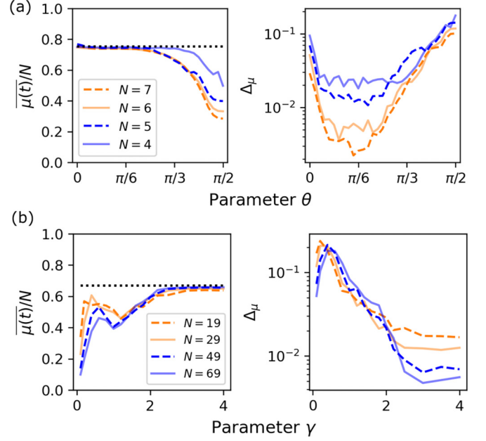
FIG. 9. System size analysis for the time-averaged mean \overline{\mu(t)} and associated temporal fluctuations \Delta_\mu for both the (a) Ising and (b) QKT models considered in the main text. Quantities are plotted as a function of the relevant parameters for each model: (a) the angle \theta between the longitudinal and transverse field for the Ising model and (b) the nonlinearity strength parameter \gamma for the QKT. Dotted lines indicate the predictions from Haar-random evolution (cf. Table I and Appendix A).
