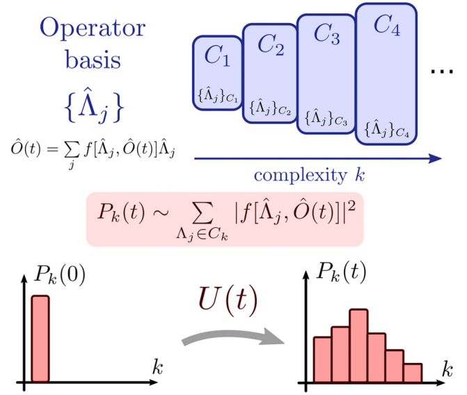
FIG. 1. Schematic picture of scrambling diagnosed via a coarse-grained operator distribution. An operator basis, typically containing exponentially many elements, is divided into sets with common characteristics C_1, C_2 , etc. A typical example of this is the size or weight of a multibody Pauli operator in the case of spin- \frac{1}{2} particles. From this grouping, a probability distribution is defined for the evolution of an operator \hat{O}(t) . At t = 0 , the distribution is localized at low complexity index. The scrambling process generated by U(t) spreads the distribution and shifts it towards higher complexity.
