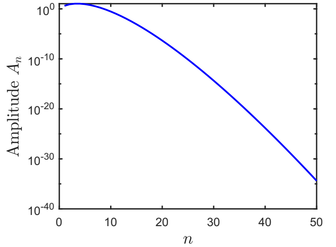
FIG. 10. Amplitude A_n of the s(\hat{Q})^n term, as defined in Eq. (D6), visualized as a function of n . We observe that the amplitude is nonzero for all n considered here, albeit exponentially decreasing. This demonstrates numerically that the polynomial (D5) is indeed order n as desired for n = 1, 2, \dots, 50 .
