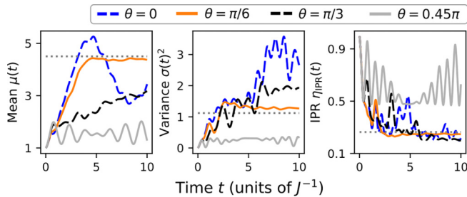
FIG. 8. Measures of the probability distribution \{P_k\} for the tilted-field Ising model with N = 6 , B/J = 1 , and \hat{O}(0) = \hat{\sigma}_y^{(1)}/\sqrt{2} .
