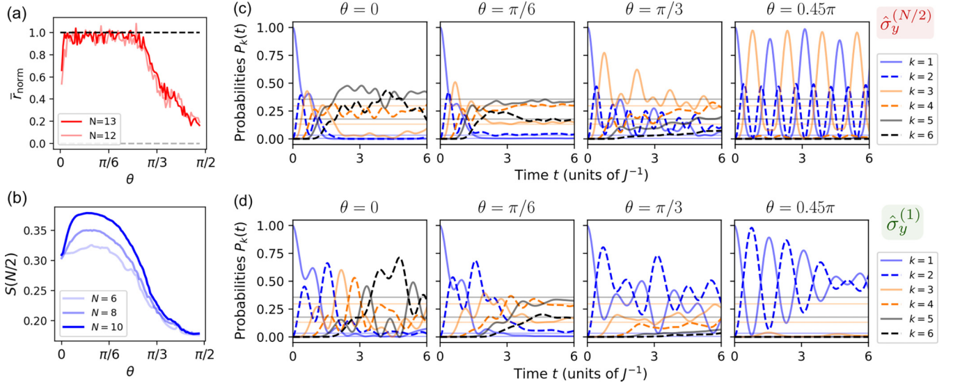
FIG. 2. Scrambling from operator evolution and quantum chaos indicators in the tilted field Ising model defined in Eq. (18), as a function of the external field angle \theta . All cases use B = J . (a) Normalized mean adjacent level spacing ratio, a standard measure of quantum chaos discussed in Appendix B, computed for two instances of the Ising Hamiltonian with different system size N . (b) Alternative proxy for quantum chaos given by the averaged entanglement entropy of the eigenstates of H_{\text{Ising}} located in the bulk of the spectrum. (c) and (d) Short-time evolution of the coarse-grained operator distribution P_k(t) , defined in Eq. (11), for different values of \theta and with N = 6 . Cases shown correspond to (c) \hat{O}(0) = \hat{\sigma}_y^{(N/2)}/\sqrt{2} and (d) \hat{O}(0) = \hat{\sigma}_y^{(1)}/\sqrt{2} . Thin faint lines indicate the values of the Haar-random evolution, given in Eqs. (8) and (10). From left to right, cases corresponding to different values of \theta \in [0, \pi/2) are shown.
