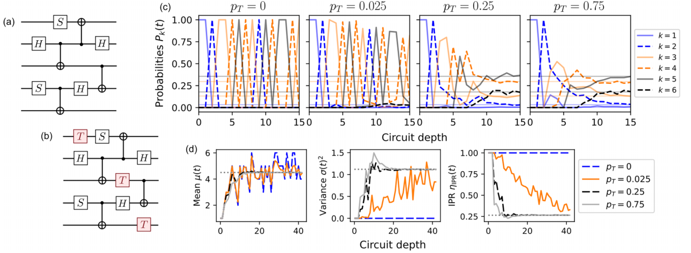
FIG. 7. Scrambling and operator growth in a random quantum circuit. (a) One instance of a random circuit composed only of the Clifford gates H , S , and CX ( p_T = 0 ). (b) Same instance with non-Clifford T gates interleaved in random locations. (c) Evolution of the operator distribution probabilities P_k(t) for different values of the T -gate probability p_T . From the left to right the “non-Cliffordness” of the circuit increases with p_T . Results shown for p_T > 0 are averages over 40 random instances. (d) Evolution of the mean \mu(t) , variance \sigma^2(t) , and IPR of the operator distribution \eta_{\text{IPR}}(t) as a function of time and for the same values of p_T as used in (c). The initial operator is \hat{O}(0) = \sigma_z^{(1)}/\sqrt{2} .
