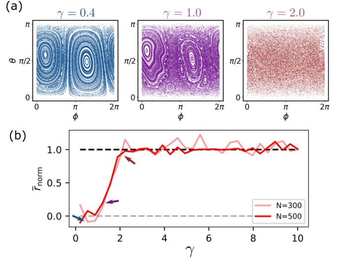
FIG. 4. Quantum and classical chaos in the kicked top model of Eq. (22), with the parameters \alpha_x = 1.7 , \alpha_y = 1 , \alpha_z = 0.8 , \gamma_x = 0.85\gamma , \gamma_y = 0.9\gamma , and \gamma_z = \gamma . (a) Phase-space portraits (Poincaré sections) of the classical kicked top for different values of the nonlinearity parameter \gamma . The system transitions from a regular regime at small \gamma to a mixed phase space for \gamma \sim 1 to a full chaotic regime for \gamma \gtrsim 2 . (b) Normalized mean adjacent level spacing ratio for two instances of the QKT with different N = 2J . Note that, due to the lack of time-reversal symmetry of this model, the measure is normalized to give 1 when the circular unitary ensemble value is achieved. See Appendix B for more details.
