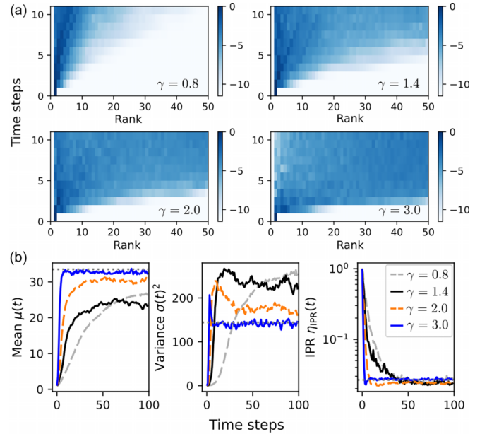
FIG. 5. Dynamics of the operator distribution for the QKT of Eq. (22). Results were obtained using parameter values for \{\alpha_i, \gamma_i\} identical to Fig. 4, N = 2J = 49 , and the initial operator \hat{O}(0) = \hat{J}_z . (a) Density plots of the operator distribution P_k(t) , shown in logarithmic scale for clarity. The quantity plotted is \log[P_k(t) + \epsilon] , with \epsilon = 10^{-10} . (b) Measures of the distributions shown in (a), calculated as a function of time.
