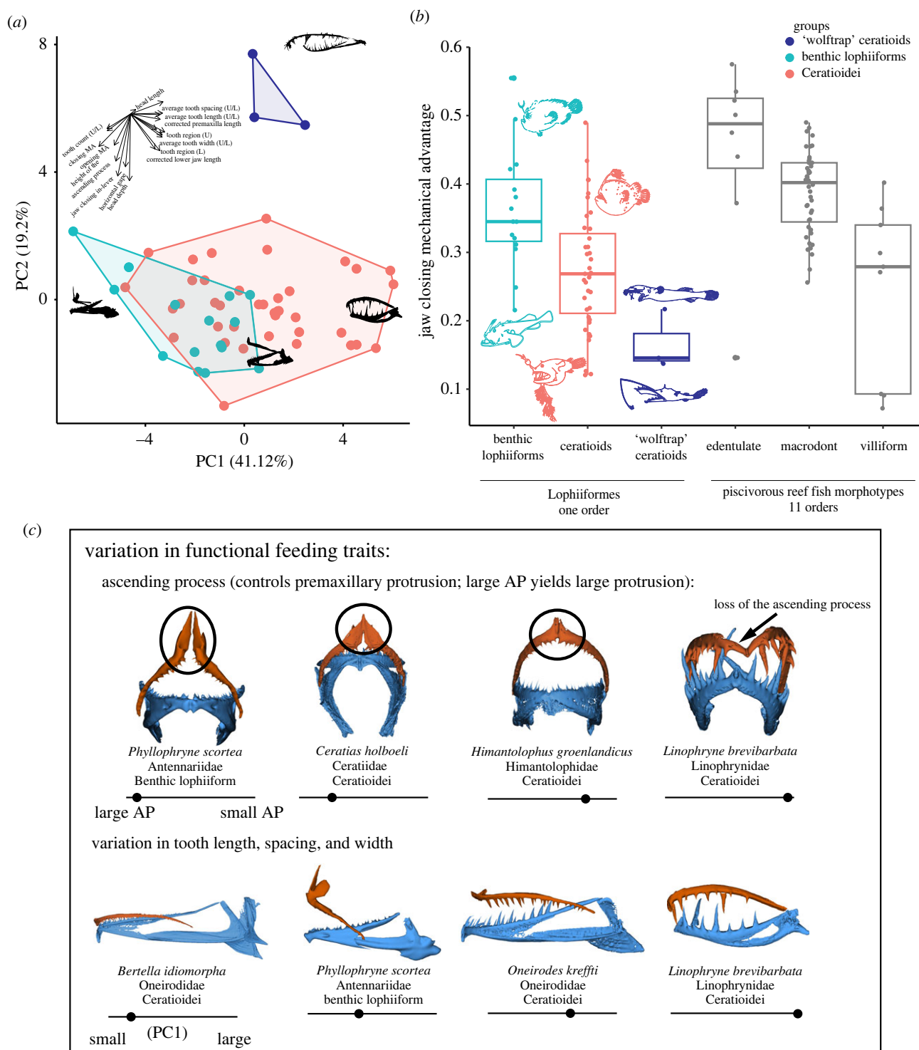
Figure 1. (a) PCA of jaw and tooth morphologies for 57 species of Lophiiformes. For pPCA, see electronic supplementary material, figure S5. (b) Mechanical advantage values measured for anglerfishes compared to morphotypes from [41]. Fish icons were digitized from FAO identification guides. (c) Examples of variation in trophic morphologies among Lophiiformes, where orange = upper jaw and blue = lower jaw. The bars below the jaws reflect the species' relative position with respect to ascending process height (top row; y-axis of figure 2b) or tooth length, spacing and width (bottom row; PC1 of (a)). Images not to scale.
