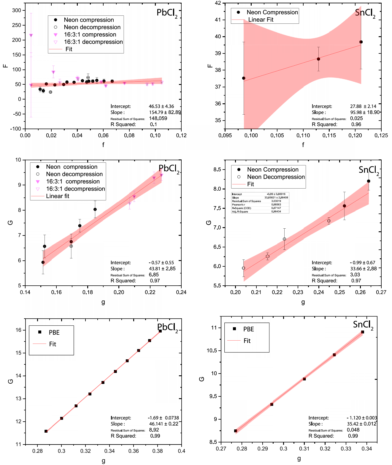
FIG. 8. Eulerian strain vs normalized strain ( F vs f ) (cotunnite phase, top) and effective strain vs normalized strain ( G vs g ) ( Co_2Si phase, middle and Co_2Si -like phase, bottom) are shown for PbCl_2 (left) and SnCl_2 (right). F vs f plots were used to determine the equations of state for the low-pressure phases, while G vs g was used for high-pressure phases [47]. Data from the phase-transition zone fit neither equation of state and were thus omitted. A weighted least-squares fit was applied to each dataset (red lines) and 95% confidence intervals are shown (red shading).
