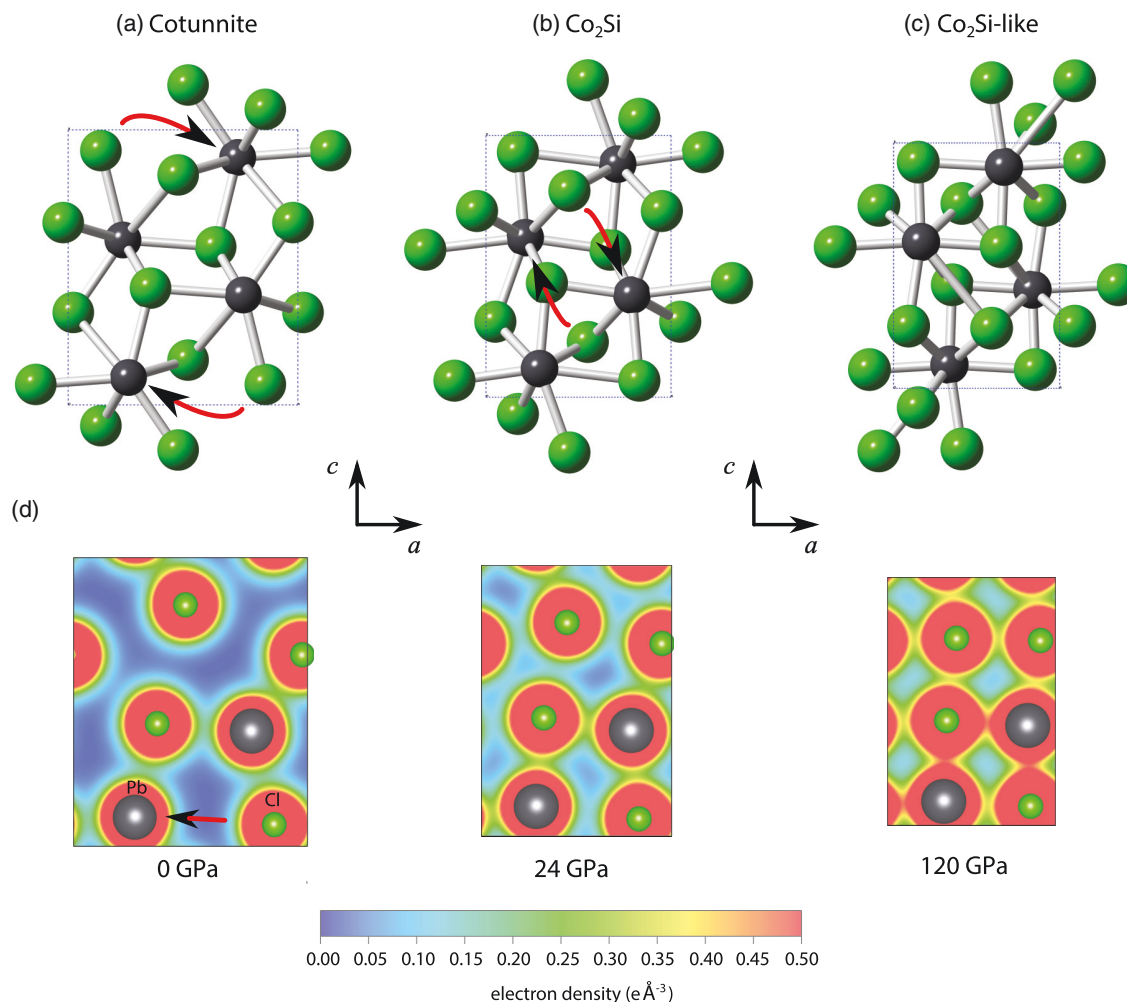
FIG. 4. Structural diagrams of the cotunnite, \text{Co}_2\text{Si} , and \text{Co}_2\text{Si} -to- \text{Co}_2\text{Si} -like phases, with the Pb, Sn cations shown in black and chlorine shown in green. (a)–(c) show ball-and-stick models of the cotunnite, \text{Co}_2\text{Si} , and \text{Co}_2\text{Si} -like structures, respectively, with arrows indicating the atomic motion that leads to bonds in subsequent phases. (d) Change in electron density in the (010) plane as a function of pressure. A bond forms between Pb and Cl at 24 GPa, indicative of a transformation from the ninefold-coordinated cotunnite structure (a) to the tenfold-coordinated \text{Co}_2\text{Si} structure (b). For \text{SnCl}_2 , formation of an analogous Sn-Cl bond is observed at about 28 GPa. On further compression the lattice continues to become more ideally packed, and (Pb,Sn)-Cl bonds form. This \text{Co}_2\text{Si} -like structure is predicted by DFT to occur at 120 GPa in \text{PbCl}_2 and 80 GPa in \text{SnCl}_2 . Figures were produced using VESTA3 [50].
