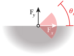
Figure 3. Schematic of the domain of possible load cases in red and the load vector basis in white ( F_x ) and black ( F_y ), with a limited range of angles ( \theta_r ), for case 2.
