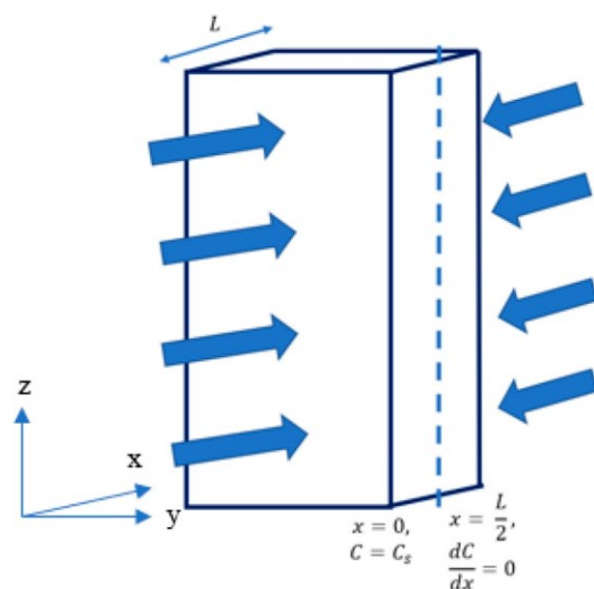
Figure 2. Sample diagram with boundary conditions.
