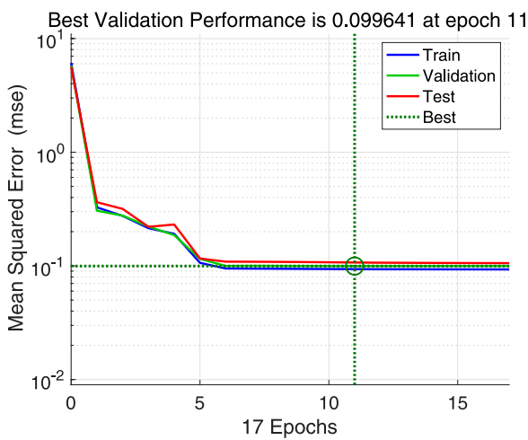
FIGURE 8 Performance of gust speed prediction using the NARXNET.
