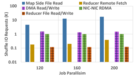
Fig. 14. Num. shuffle I/O reqs for the join op in TPC-H Q13.
