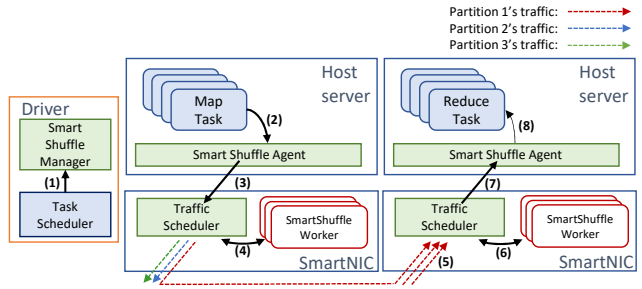
Fig. 5. SmartShuffle Overview
