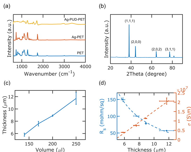
Figure 2. Chemical and structural characterization of cured Ag films. (a) FTIR for PET, Ag-PET, and Ag-PUD-PET, respectively, and (b) XRD for Ag-PUD-PET. (c) Thickness of Ag layer from SEM for different volume coated Ag-PUD-PET. (d) Sheet resistance and electric conductivity at different thicknesses.
