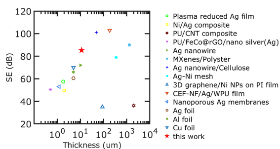
Figure 4. Comparison of EMI SE and thickness between our work to Plasma Ag deposition, 18 Ni/Ag composite, 14 PU/CNT composite, 40 PU/FeCo@rGO, 41 Ag nanowire, 11 MXenes/Polyster, 22 Ag nanowire/cellulose, 23 Ag–Ni mesh, 21 3D graphene with Ni NPs, 21 CEF-NF/Ag/WPU film, 39 nanoporous Ag membranes, 42 Ag foil, 42 and Cu foil. 42
