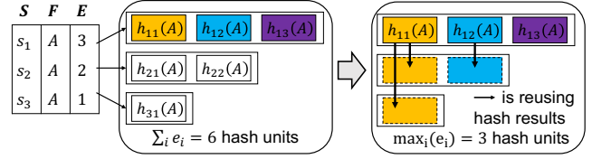
Figure 4: HASHREUSE ( O_{Hash1} ) reduces hash units by reusing hash results. A small box with h_{seed}(\text{flowkey}) indicates one hash unit allocation.
