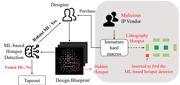
Figure 1: Malicious IP vendors may use adversarial perturbations to hide hotspots in immature designs. Designers using an unrobust ML-based hotspot detector for printability verification may suffer from great loss at the tapeout stage due to hidden hotspots.
