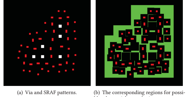
Figure 3: Illustration of via and SRAF patterns of a given layout and its corresponding regions for possible adversarial perturbations. In (a), the red rectangles denote existing SRAFs, and the white squares denote vias. In (b), the green region denotes the DRC-clean fraudulent SRAF insertion spots. And the red rectangles denote the adversarial removal candidates, which correspond to the preexisting SRAFs.
