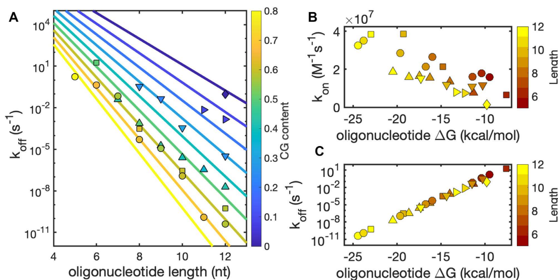
Figure 4. Kinetics of dissociation and association of short RNA oligonucleotides. k_{on} was measured as previously described in this work, while k_{off} was calculated as k_{on} \cdot K_D . (A) k_{off} for the oligonucleotides studied in this work as a function of length shows a poor correlation and emphasizes the dramatic scaling and role of CG content. Straight lines are predictions calculated from Equations (9) and (10). (B) k_{on} as a function of \Delta G shows a linear dependence. (C) k_{off} as a function of \Delta G shows a strong exponential correlation.
