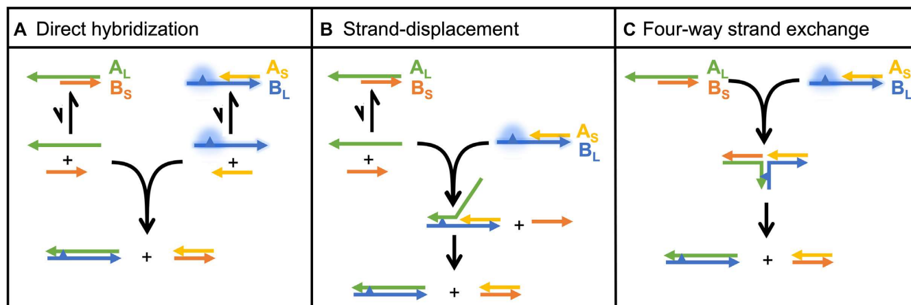
Figure 7. Equilibration pathways expected to determine the evolution of A_S B_L in complex mixtures of competing oligonucleotides.
