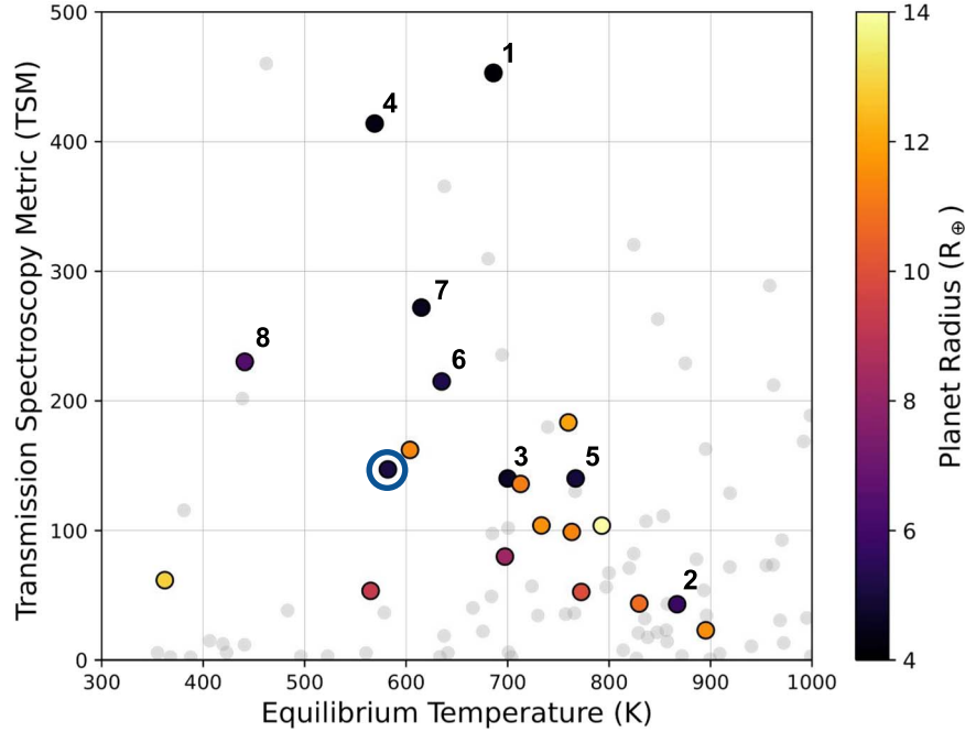
Figure 6. The TSM of known exoplanets with both a measured ( >3\sigma ) mass and radii >4 R_{\oplus} as a function of equilibrium temperature. Planets orbiting M dwarfs are labeled according to Table 6 and are noted with colors varying by their respective planetary radii, while planets orbiting FGK-dwarf stars are plotted as gray points. TOI-3785 b (navy blue circle) possesses one of the highest TSMs for any planet cooler than 600 K, making it a promising target for future transmission spectroscopy observations.
