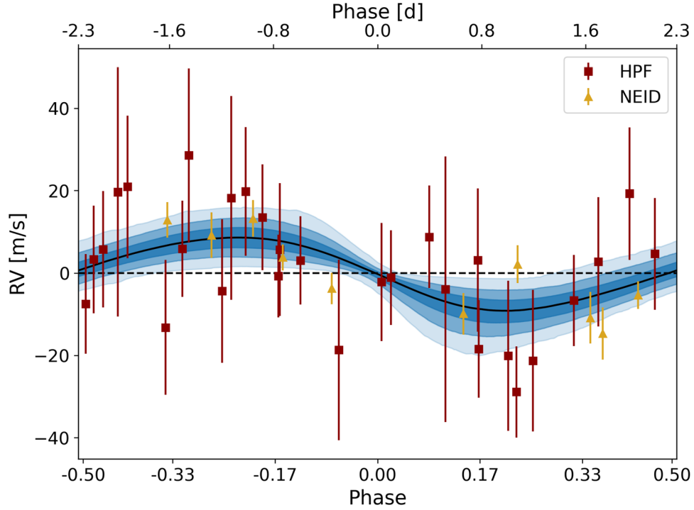
Figure 3. Phase-folded RV points from both HPF (dark red) and NEID (gold) with the best-fit model plotted in blue along with the 1, 2, and 3\sigma contours (similar to Figure 1) generated from the exoplanet joint fit.
