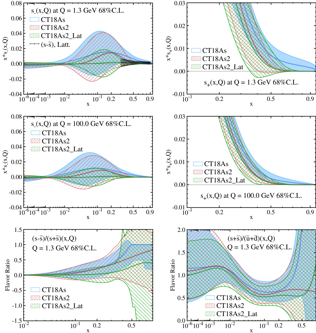
FIG. 20. The comparison of s_-(x) , and s_+(x) PDFs at the initial Q_0 (= 1.3 GeV) scale and Q = 100 GeV, as well as PDF ratio (s - \bar{s})/(s + \bar{s})(x) and (s + \bar{s})/(\bar{u} + \bar{d})(x) at Q_0 = 1.3 GeV, for CT18As, CT18As2, and CT18As2_Lat.
