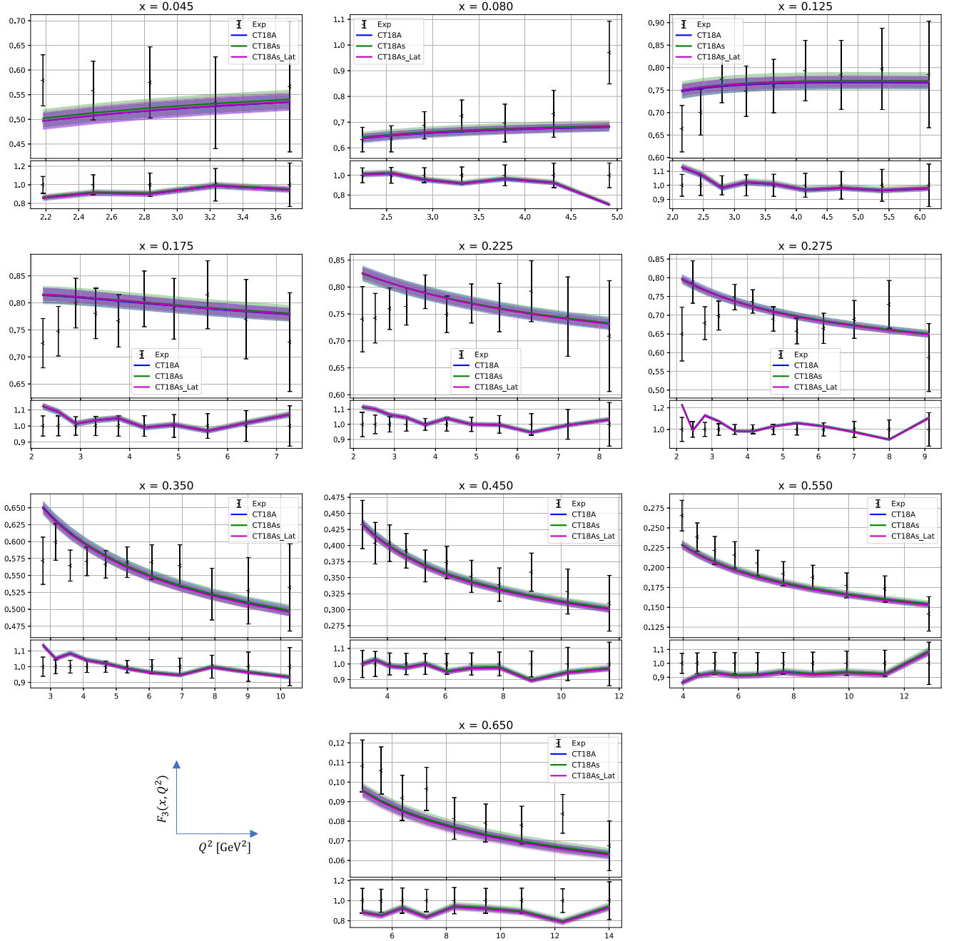
FIG. 11. Comparison of data and theories for the CDHSW F_3^p structure function measurements [41] (ID = 109). The unshifted data are presented in the form of F_3 as a function of Q^2 for a certain values of x .
