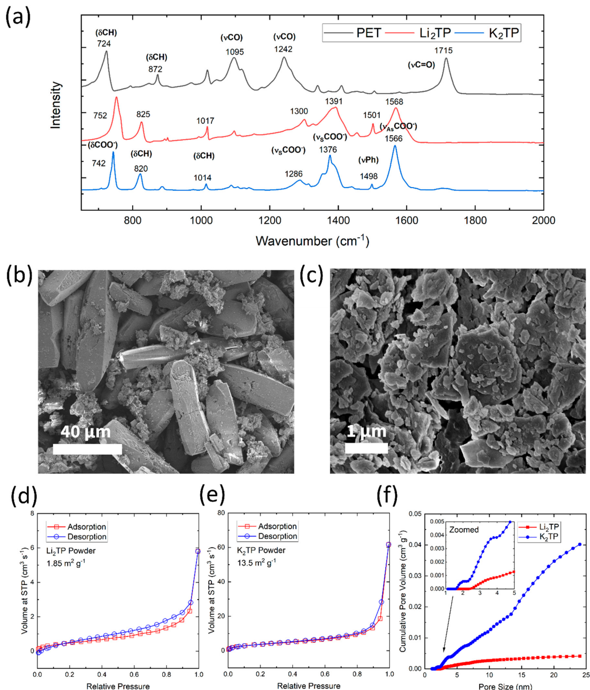
Figure 2. Characterizations of starting materials including (a) FTIR spectra of the PET bottle flakes, Li 2 TP, and K 2 TP, as well as SEM images of the synthesized (b) Li 2 TP and (c) K 2 TP powders. Characterization also includes nitrogen adsorption/desorption isotherms with calculated BET surface area for (d) Li 2 TP and (e) K 2 TP, as well as (f) calculated pore size distributions for both TPS.
