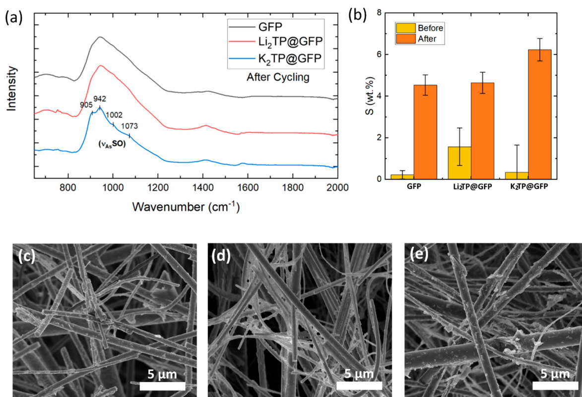
Figure 5. Post-mortem analysis of modified and unmodified separators cycled in LSBs including (a) FTIR, (b) EDS sulfur quantitative analysis, and SEM of (c) GFP, (d) Li 2 TP@GFP, and (e) K 2 TP@GFP.
