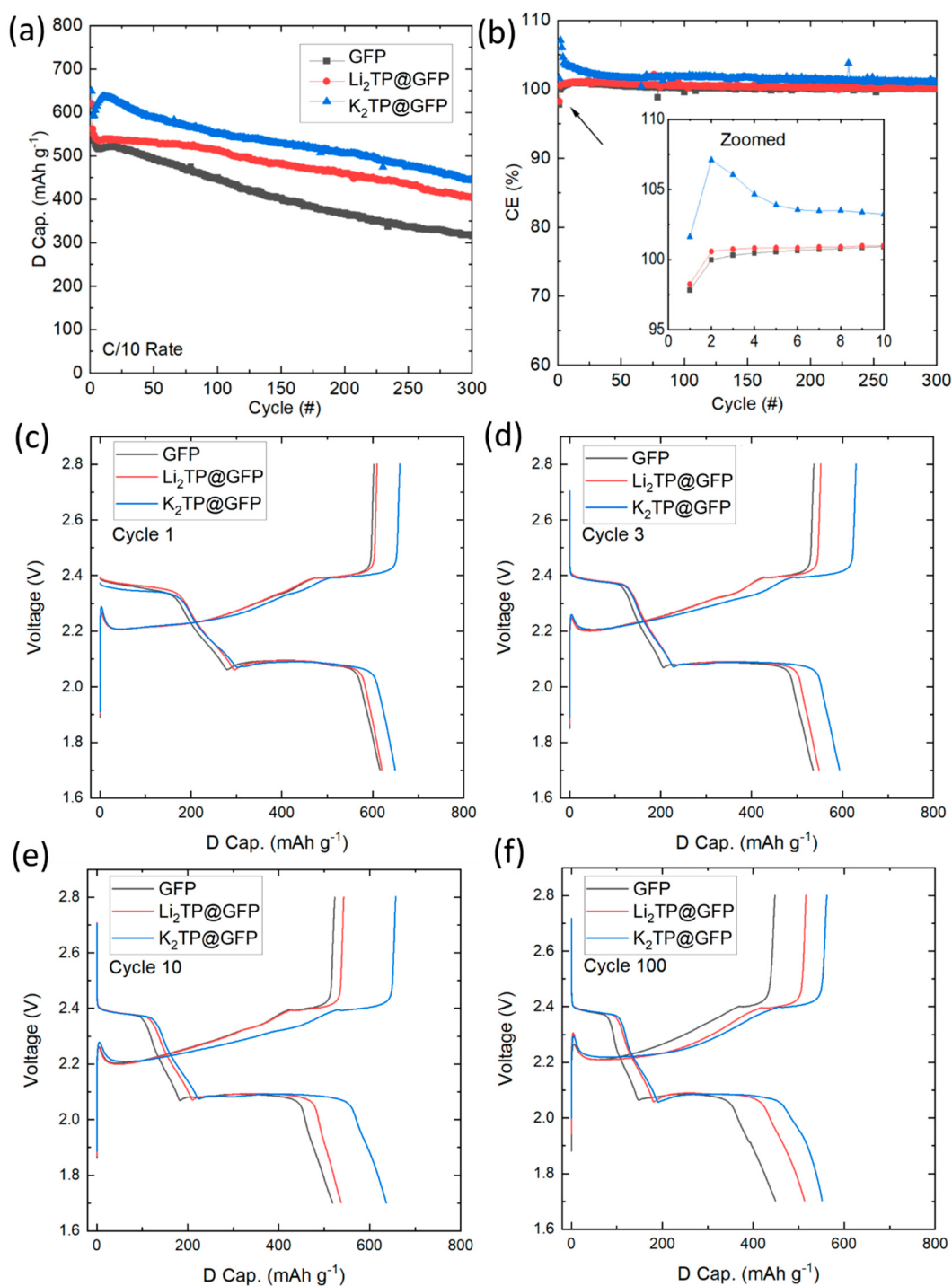
Figure 4. (a) C/10 cycling and (b) CE of LSBs with modified and modified separators, as well as select voltage profiles from cycles (c) 1, (d) 3, (e) 10, and (f) 100.
