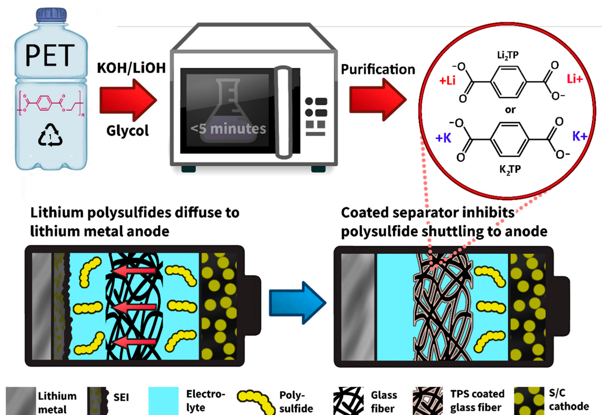
Figure 1. Pictorial of synthetic process of TPS from waste PET and LiPS blocking mechanism of the modified separator.
