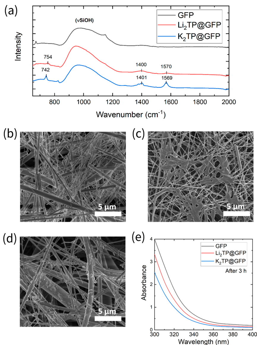
Figure 3. Characterizations of separators, including (a) FTIR spectra of modified and unmodified GFP, as well as SEM images of (b) GFP, (c) \text{Li}_2\text{TP@GFP} , and (d) \text{K}_2\text{TP@GFP} . (e) Absorbance spectra of DOL:DME solution after 3 h against 0.1 M \text{Li}_2\text{S}_6 solution in separator diffusion test.
