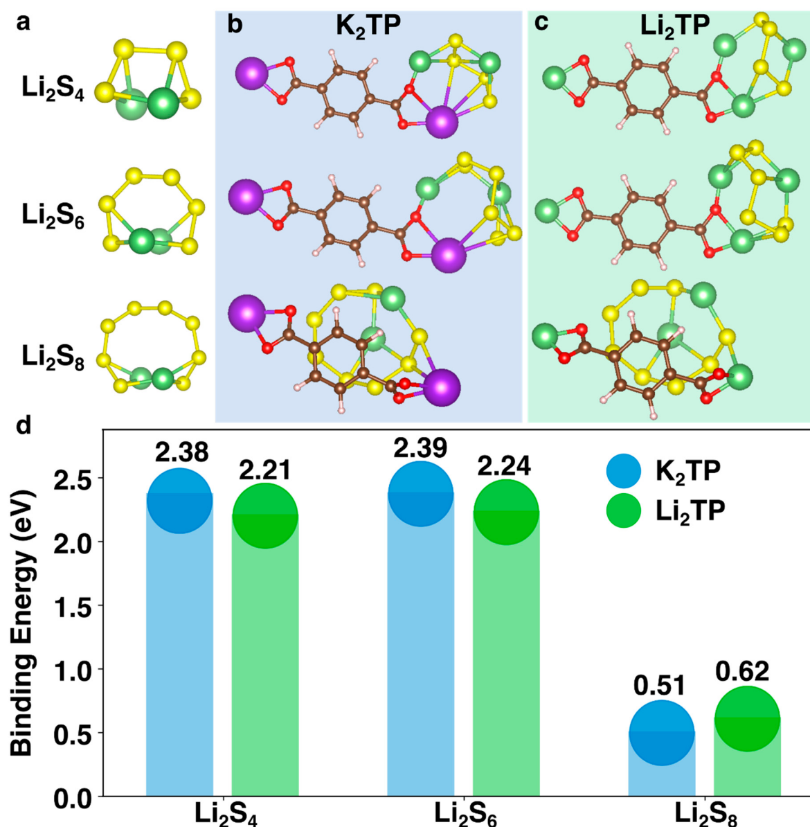
Figure 6. Binding energy between \text{Li}_2\text{TP} and \text{K}_2\text{TP} , and \text{Li}_2\text{S}_4 , \text{Li}_2\text{S}_6 , and \text{Li}_2\text{S}_8 . (a) optimized geometry of \text{Li}_2\text{S}_4 , \text{Li}_2\text{S}_6 , and \text{Li}_2\text{S}_8 ; binding configurations for (b) \text{K}_2\text{TP} -LiPSs and (c) \text{Li}_2\text{TP} -LiPSs; (d) summary of binding energy for each TPS-LiPS pair. The atoms were colored as: Li, green; K, purple; S, yellow; C, brown; O, red.
